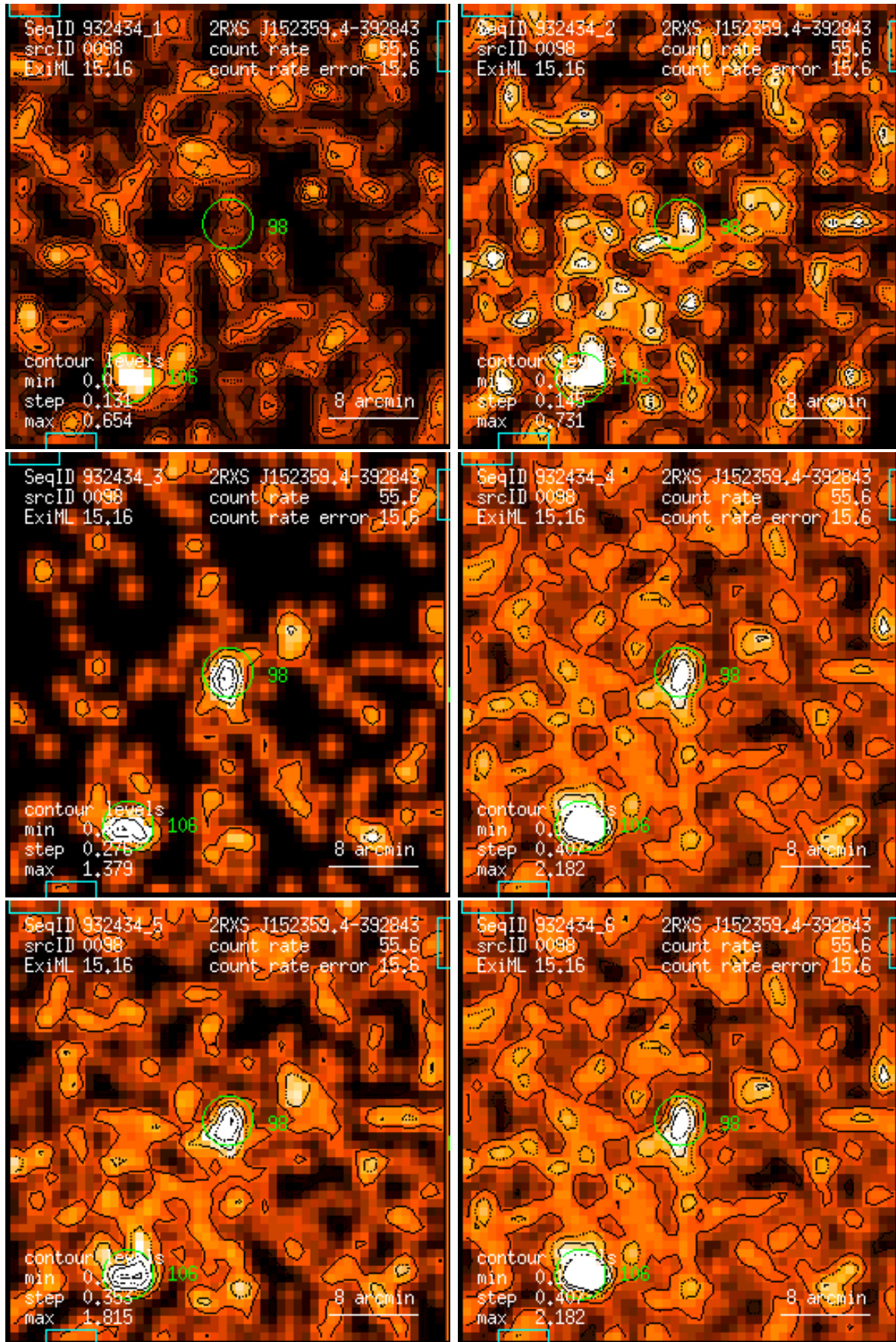
Figure 98: RASS 932434: detection 0098: band rate images, Gaussian filter: (1) PSPC channels 11 – 41, (2) 52 – 90, (3) 91 – 201, (4) 11 – 235, (5) 52 – 201, (6) 11 – 201. Broad band rates in counts/ks. Band rate contour levels in counts/ks/arcmin 2 .
