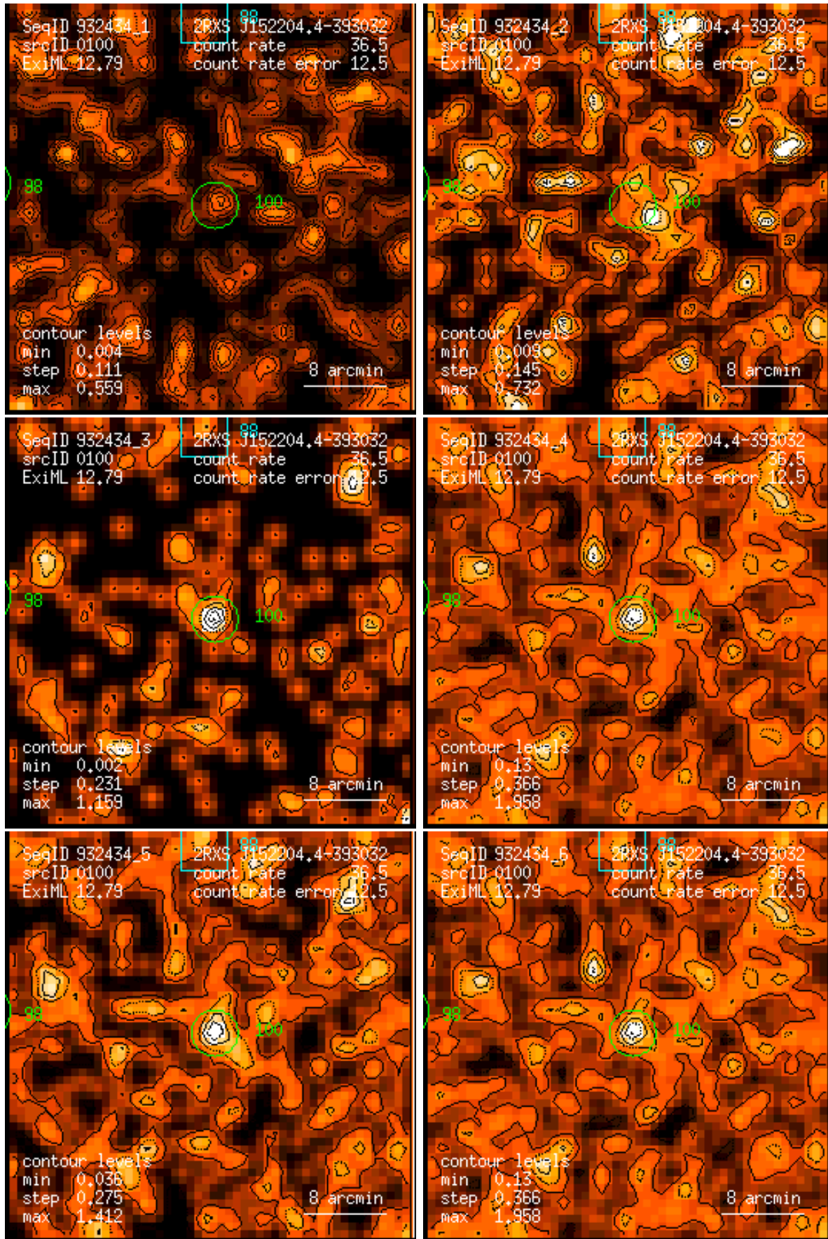
Figure 100: RASS 932434: detection 0100: band rate images, Gaussian filter: (1) PSPC channels 11 – 41, (2) 52 – 90, (3) 91 – 201, (4) 11 – 235, (5) 52 – 201, (6) 11 – 201. Broad band rates in counts/ks. Band rate contour levels in counts/ks/arcmin 2 .
