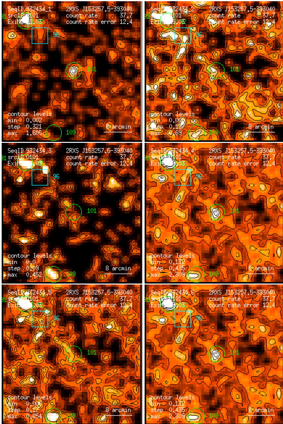
Figure 101: RASS 932434: detection 0101: band rate images, Gaussian filter: (1) PSPC channels 11 – 41, (2) 52 – 90, (3) 91 – 201, (4) 11 – 235, (5) 52 – 201, (6) 11 – 201. Broad band rates in counts/ks. Band rate contour levels in counts/ks/arcmin 2 .
