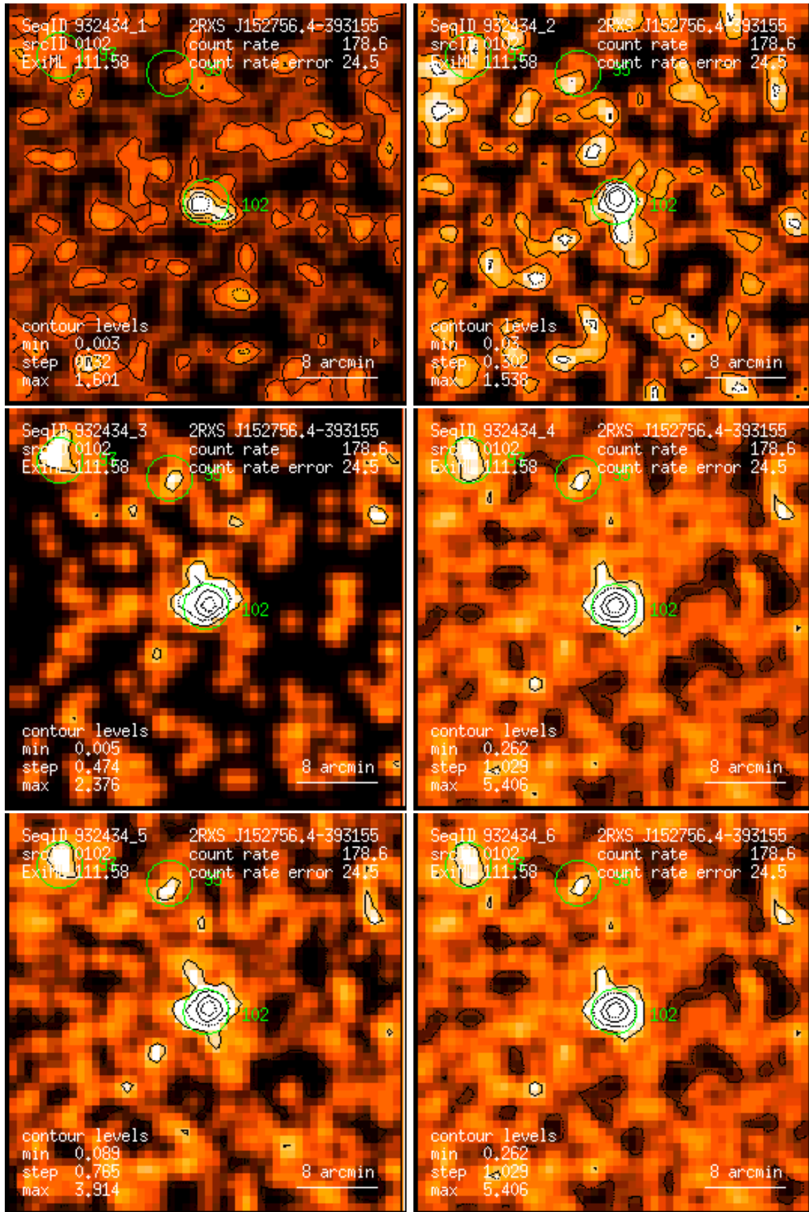
Figure 102: RASS 932434: detection 0102: band rate images, Gaussian filter: (1) PSPC channels 11 – 41, (2) 52 – 90, (3) 91 – 201, (4) 11 – 235, (5) 52 – 201, (6) 11 – 201. Broad band rates in counts/ks. Band rate contour levels in counts/ks/arcmin 2 .
