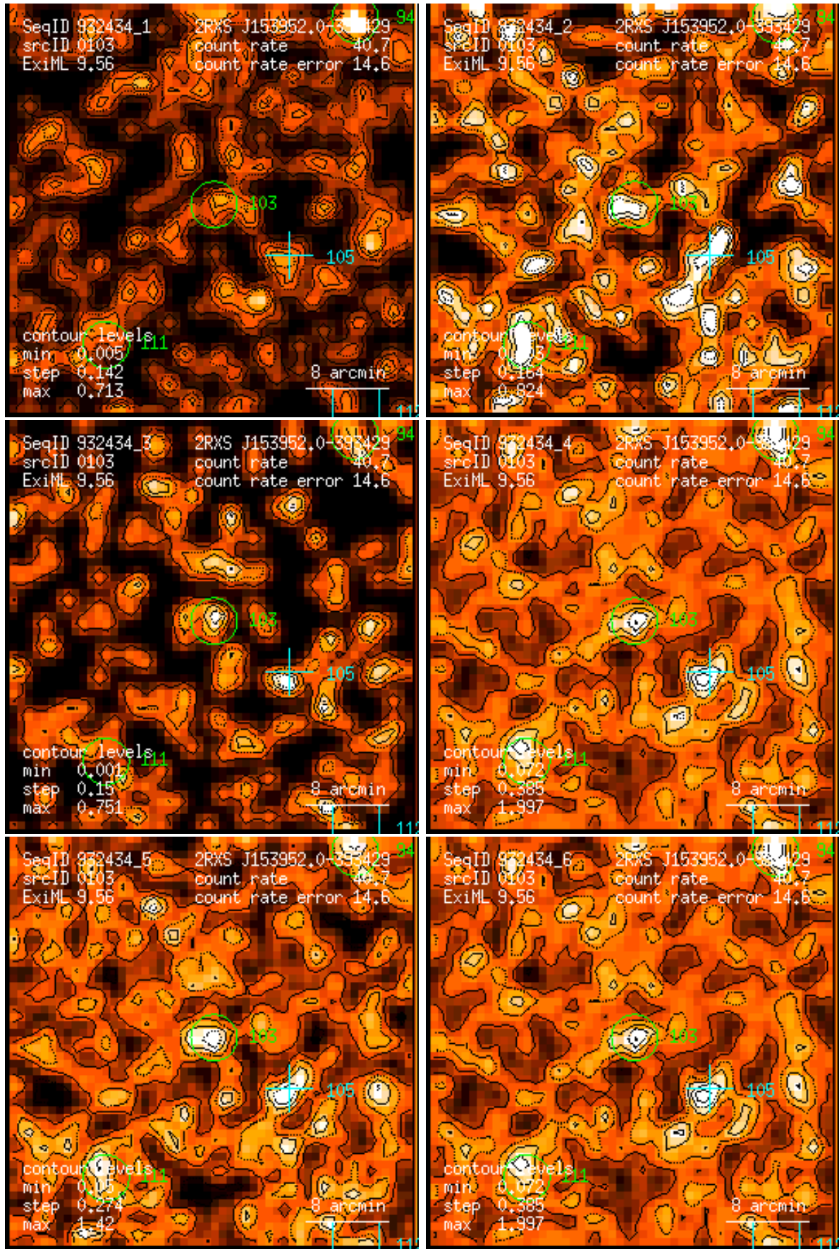
Figure 103: RASS 932434: detection 0103: band rate images, Gaussian filter: (1) PSPC channels 11 – 41, (2) 52 – 90, (3) 91 – 201, (4) 11 – 235, (5) 52 – 201, (6) 11 – 201. Broad band rates in counts/ks. Band rate contour levels in counts/ks/arcmin 2 .
