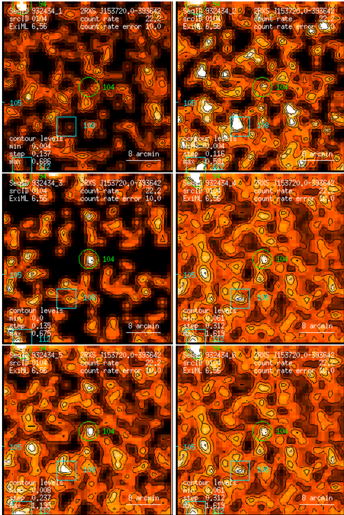
Figure 104: RASS 932434: detection 0104: band rate images, Gaussian filter: (1) PSPC channels 11 – 41, (2) 52 – 90, (3) 91 – 201, (4) 11 – 235, (5) 52 – 201, (6) 11 – 201. Broad band rates in counts/ks. Band rate contour levels in counts/ks/arcmin 2 .
