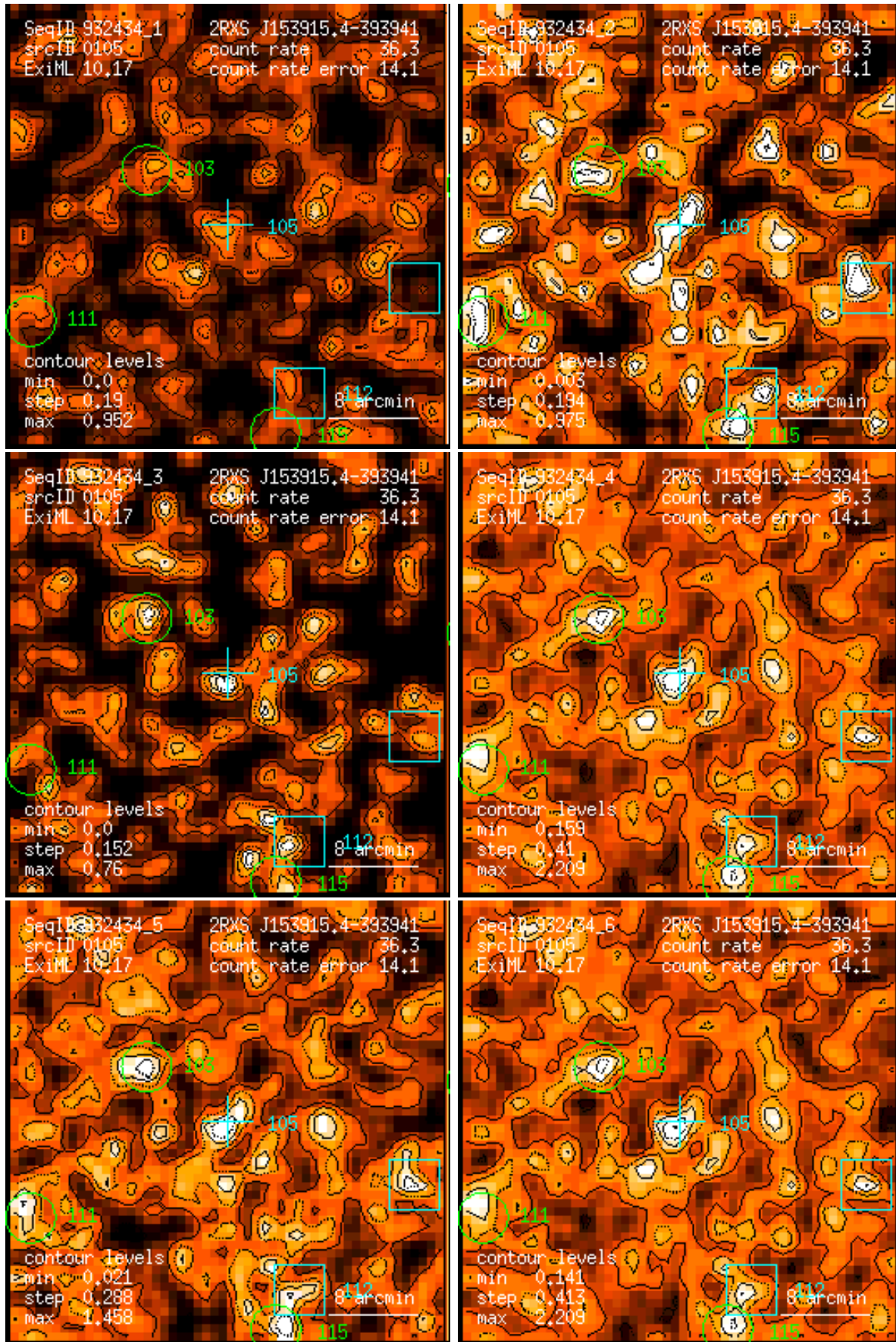
Figure 105: RASS 932434: detection 0105: band rate images, Gaussian filter: (1) PSPC channels 11 – 41, (2) 52 – 90, (3) 91 – 201, (4) 11 – 235, (5) 52 – 201, (6) 11 – 201. Broad band rates in counts/ks. Band rate contour levels in counts/ks/arcmin 2 .
