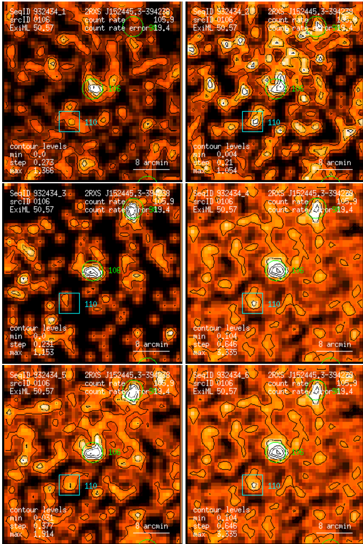
Figure 106: RASS 932434: detection 0106: band rate images, Gaussian filter: (1) PSPC channels 11 – 41, (2) 52 – 90, (3) 91 – 201, (4) 11 – 235, (5) 52 – 201, (6) 11 – 201. Broad band rates in counts/ks. Band rate contour levels in counts/ks/arcmin 2 .
