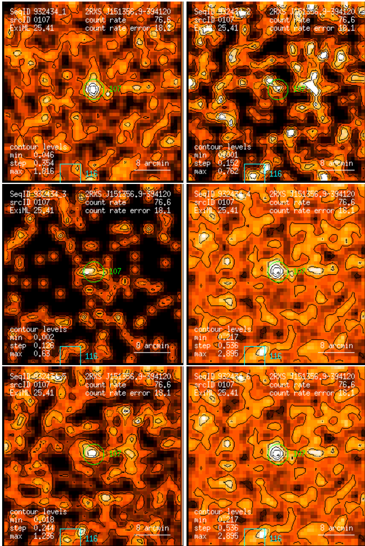
Figure 107: RASS 932434: detection 0107: band rate images, Gaussian filter: (1) PSPC channels 11 – 41, (2) 52 – 90, (3) 91 – 201, (4) 11 – 235, (5) 52 – 201, (6) 11 – 201. Broad band rates in counts/ks. Band rate contour levels in counts/ks/arcmin 2 .
