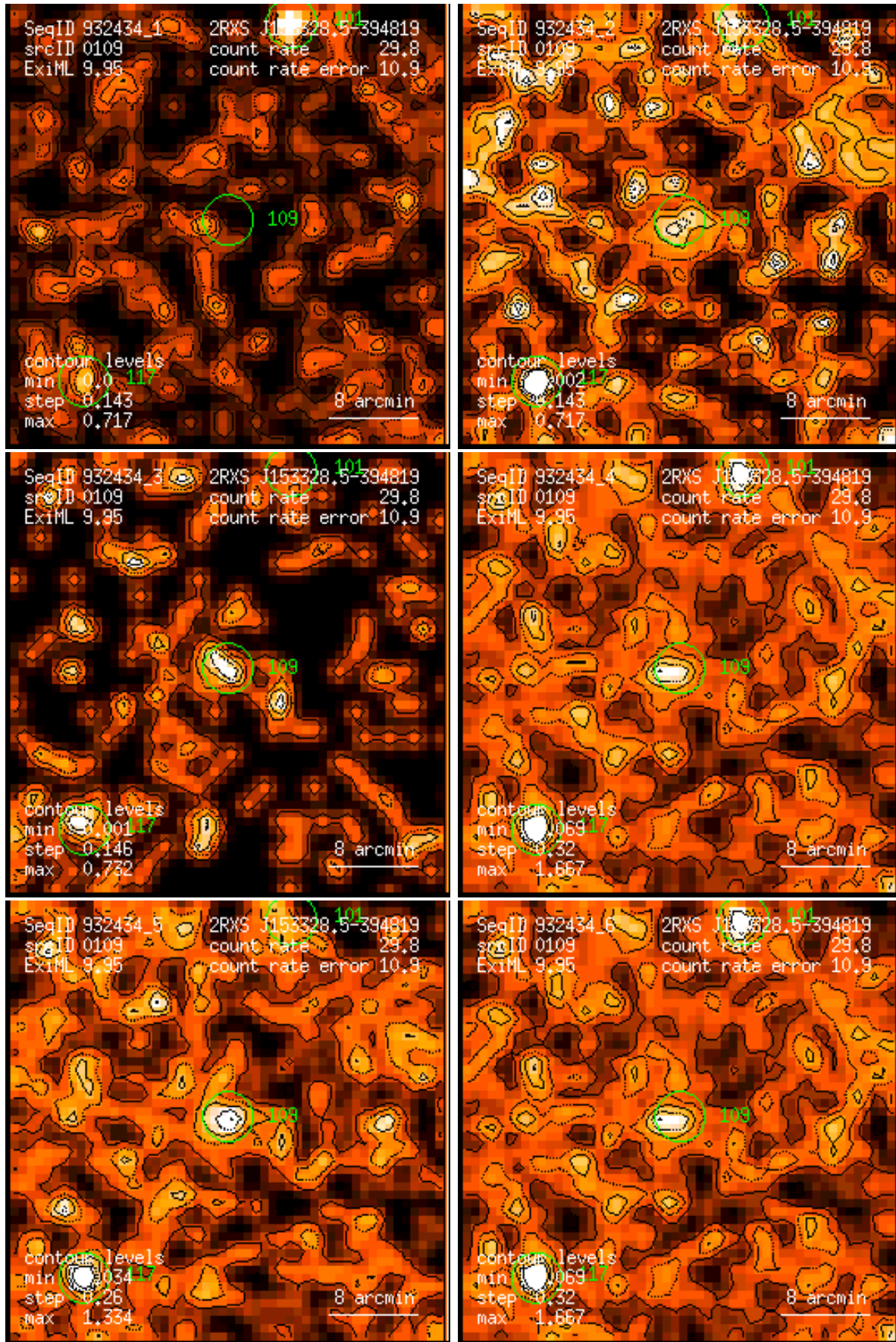
Figure 109: RASS 932434: detection 0109: band rate images, Gaussian filter: (1) PSPC channels 11 – 41, (2) 52 – 90, (3) 91 – 201, (4) 11 – 235, (5) 52 – 201, (6) 11 – 201. Broad band rates in counts/ks. Band rate contour levels in counts/ks/arcmin 2 .
