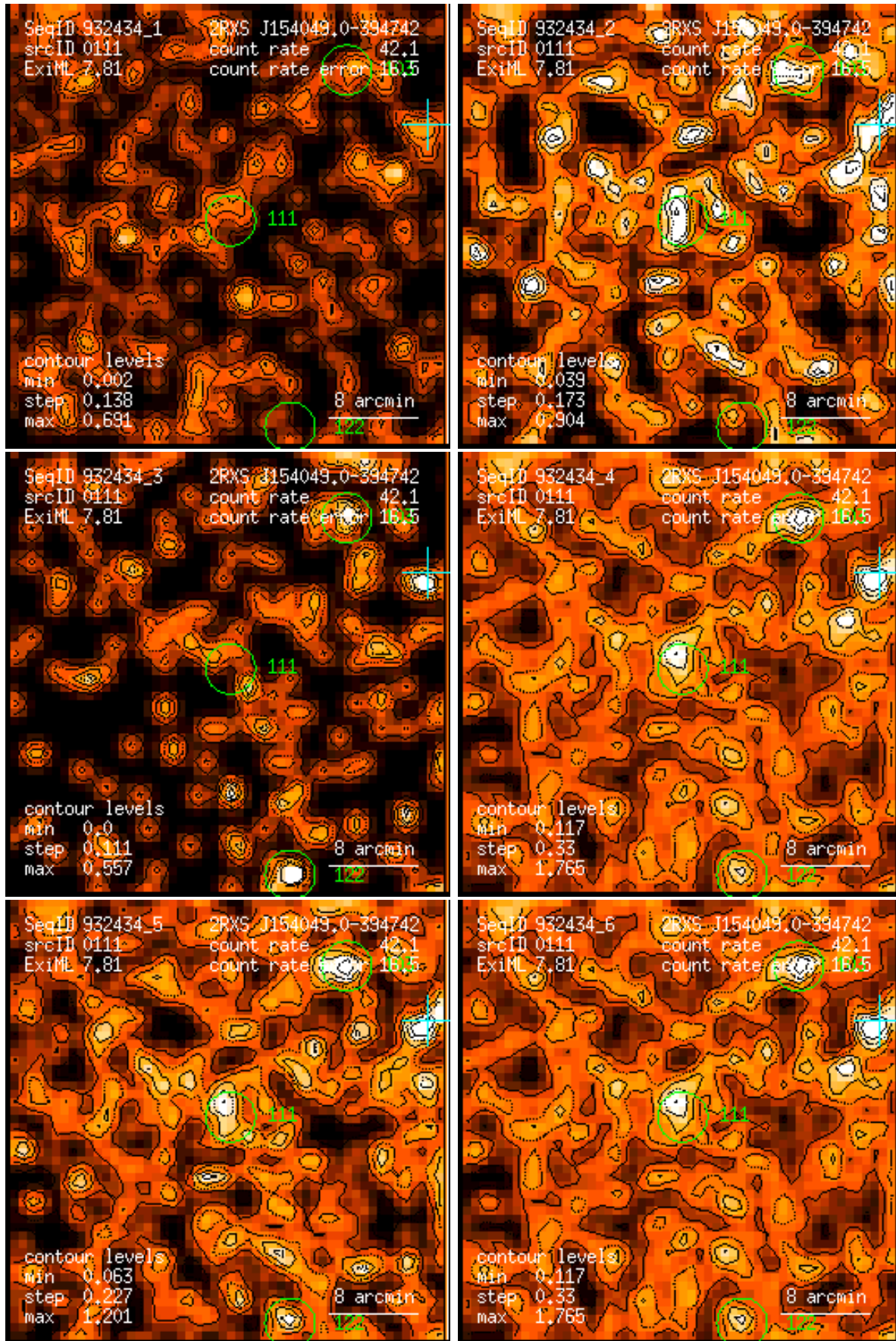
Figure 111: RASS 932434: detection 0111: band rate images, Gaussian filter: (1) PSPC channels 11 – 41, (2) 52 – 90, (3) 91 – 201, (4) 11 – 235, (5) 52 – 201, (6) 11 – 201. Broad band rates in counts/ks. Band rate contour levels in counts/ks/arcmin 2 .
