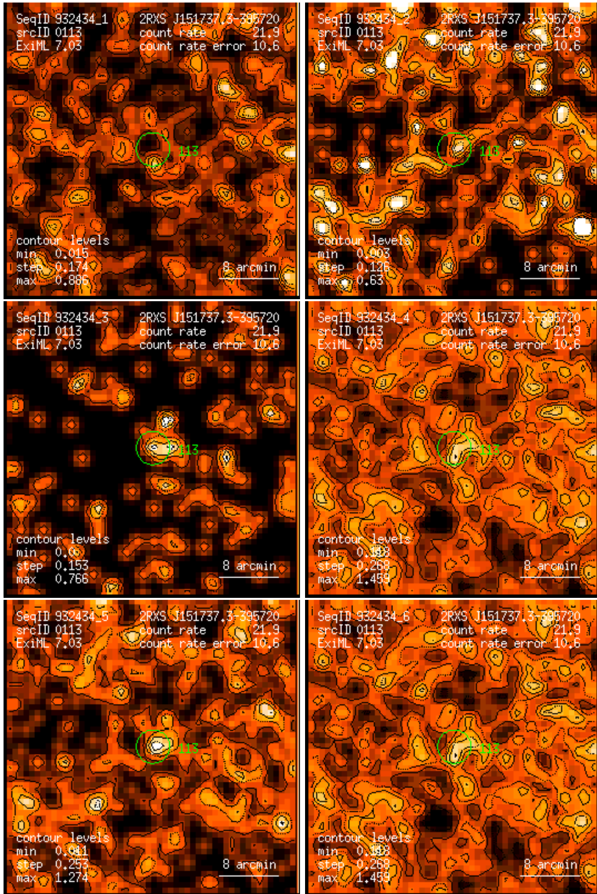
Figure 113: RASS 932434: detection 0113: band rate images, Gaussian filter: (1) PSPC channels 11 – 41, (2) 52 – 90, (3) 91 – 201, (4) 11 – 235, (5) 52 – 201, (6) 11 – 201. Broad band rates in counts/ks. Band rate contour levels in counts/ks/arcmin 2 .
