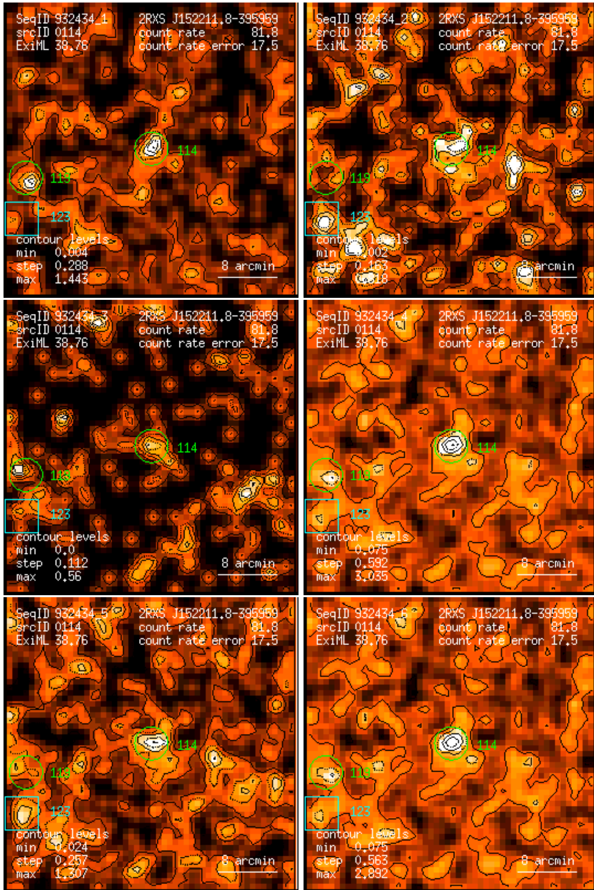
Figure 114: RASS 932434: detection 0114: band rate images, Gaussian filter: (1) PSPC channels 11 – 41, (2) 52 – 90, (3) 91 – 201, (4) 11 – 235, (5) 52 – 201, (6) 11 – 201. Broad band rates in counts/ks. Band rate contour levels in counts/ks/arcmin 2 .
