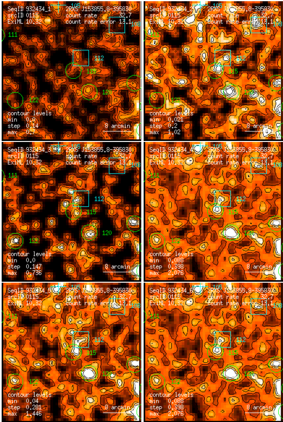
Figure 115: RASS 932434: detection 0115: band rate images, Gaussian filter: (1) PSPC channels 11 – 41, (2) 52 – 90, (3) 91 – 201, (4) 11 – 235, (5) 52 – 201, (6) 11 – 201. Broad band rates in counts/ks. Band rate contour levels in counts/ks/arcmin 2 .
