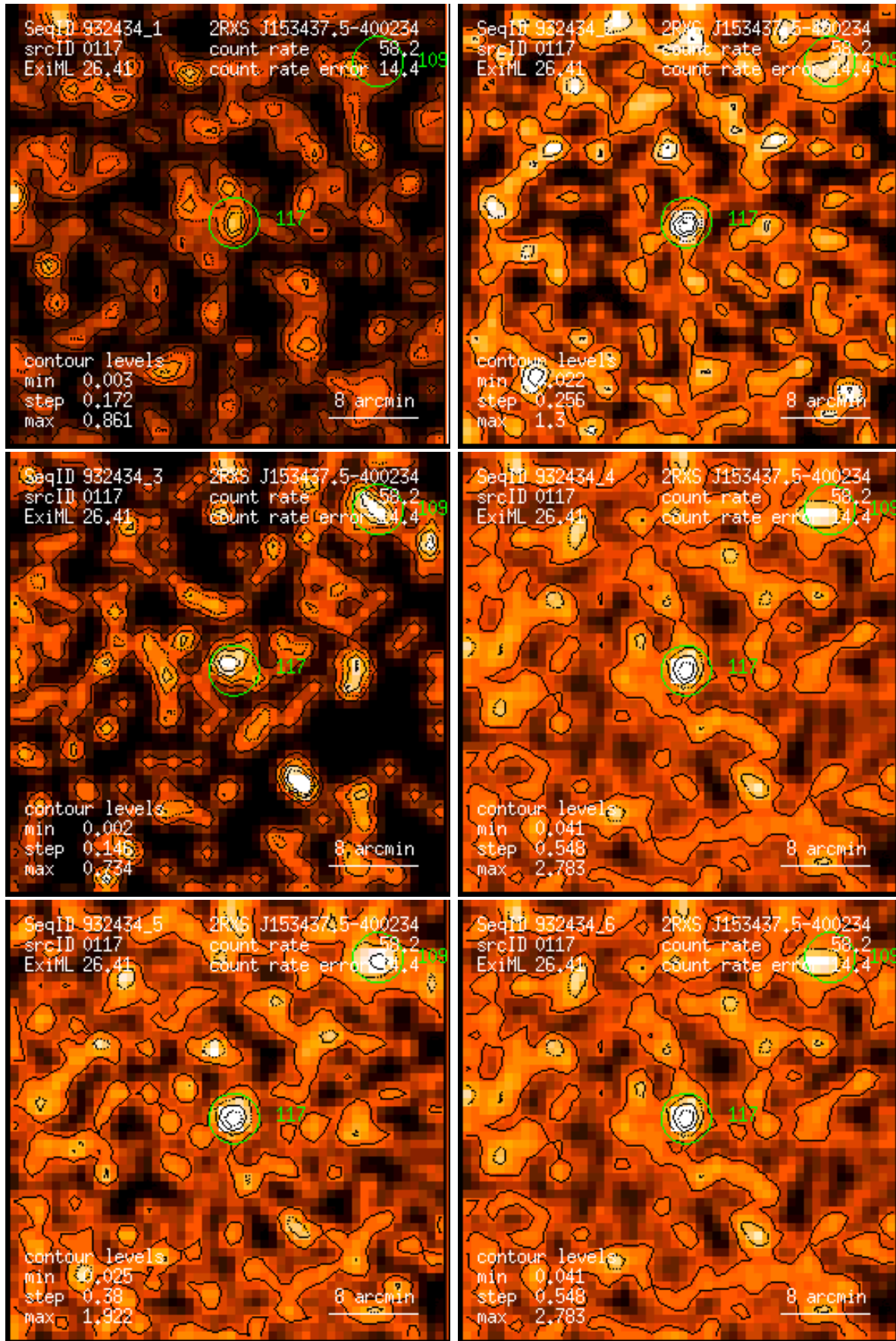
Figure 117: RASS 932434: detection 0117: band rate images, Gaussian filter: (1) PSPC channels 11 – 41, (2) 52 – 90, (3) 91 – 201, (4) 11 – 235, (5) 52 – 201, (6) 11 – 201. Broad band rates in counts/ks. Band rate contour levels in counts/ks/arcmin 2 .
