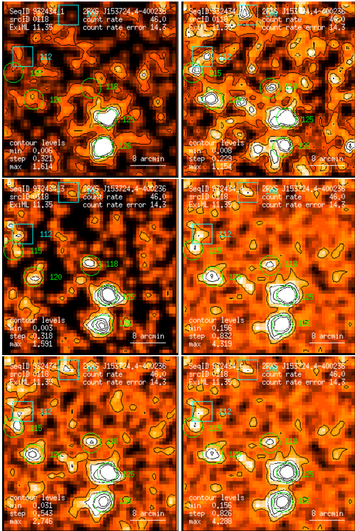
Figure 118: RASS 932434: detection 0118: band rate images, Gaussian filter: (1) PSPC channels 11 – 41, (2) 52 – 90, (3) 91 – 201, (4) 11 – 235, (5) 52 – 201, (6) 11 – 201. Broad band rates in counts/ks. Band rate contour levels in counts/ks/arcmin 2 .
