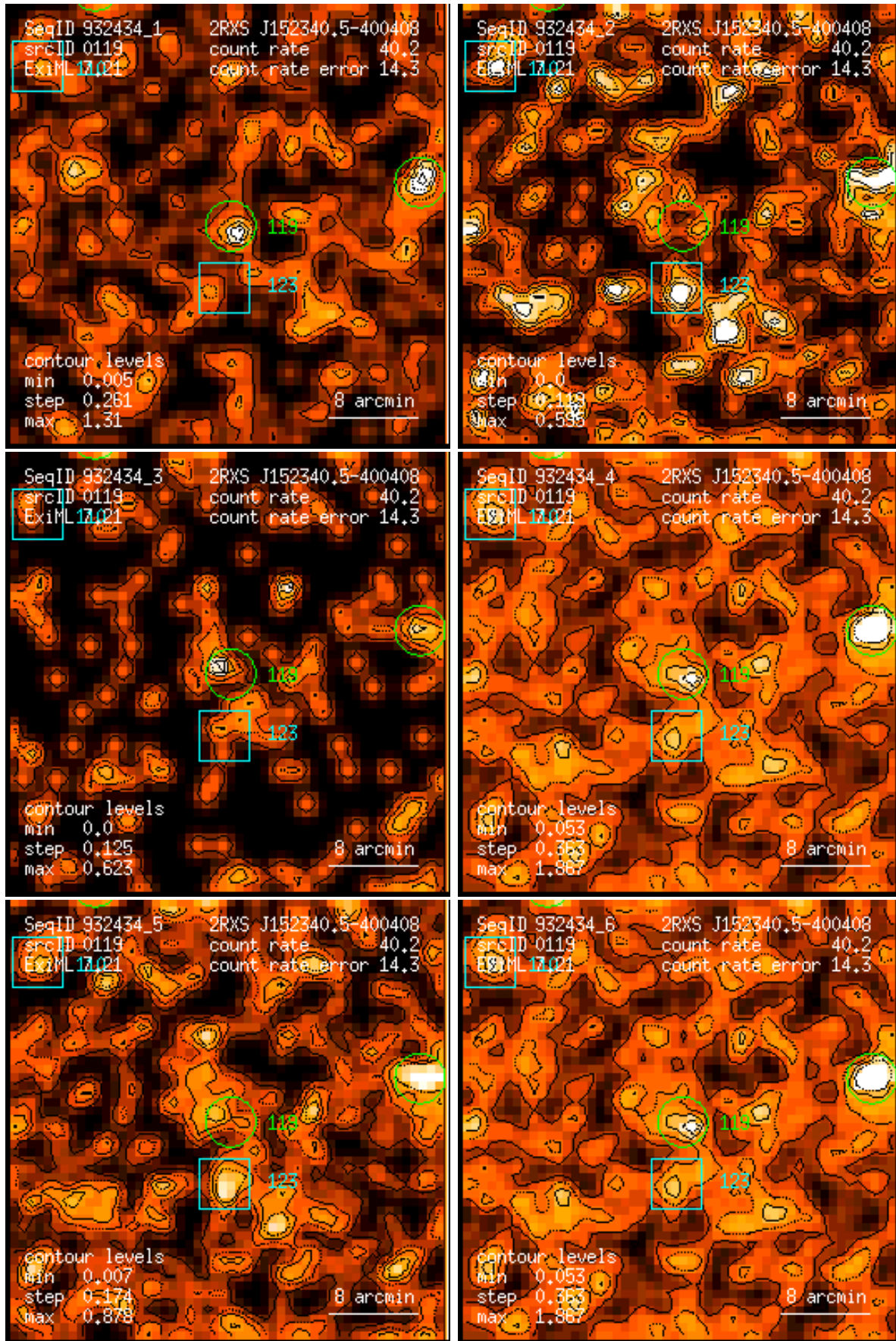
Figure 119: RASS 932434: detection 0119: band rate images, Gaussian filter: (1) PSPC channels 11 – 41, (2) 52 – 90, (3) 91 – 201, (4) 11 – 235, (5) 52 – 201, (6) 11 – 201. Broad band rates in counts/ks. Band rate contour levels in counts/ks/arcmin 2 .
