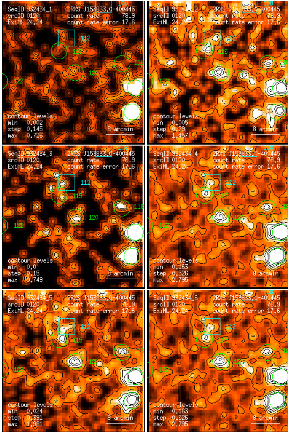
Figure 120: RASS 932434: detection 0120: band rate images, Gaussian filter: (1) PSPC channels 11 – 41, (2) 52 – 90, (3) 91 – 201, (4) 11 – 235, (5) 52 – 201, (6) 11 – 201. Broad band rates in counts/ks. Band rate contour levels in counts/ks/arcmin 2 .
