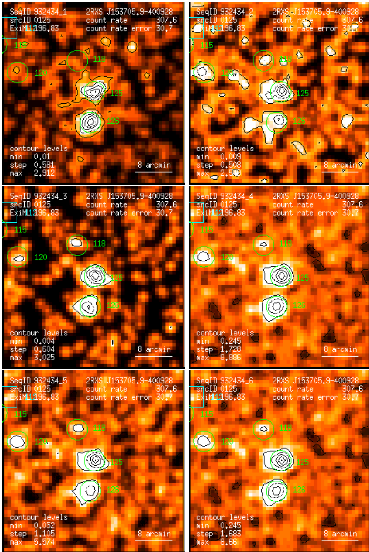
Figure 125: RASS 932434: detection 0125: band rate images, Gaussian filter: (1) PSPC channels 11 – 41, (2) 52 – 90, (3) 91 – 201, (4) 11 – 235, (5) 52 – 201, (6) 11 – 201. Broad band rates in counts/ks. Band rate contour levels in counts/ks/arcmin 2 .
