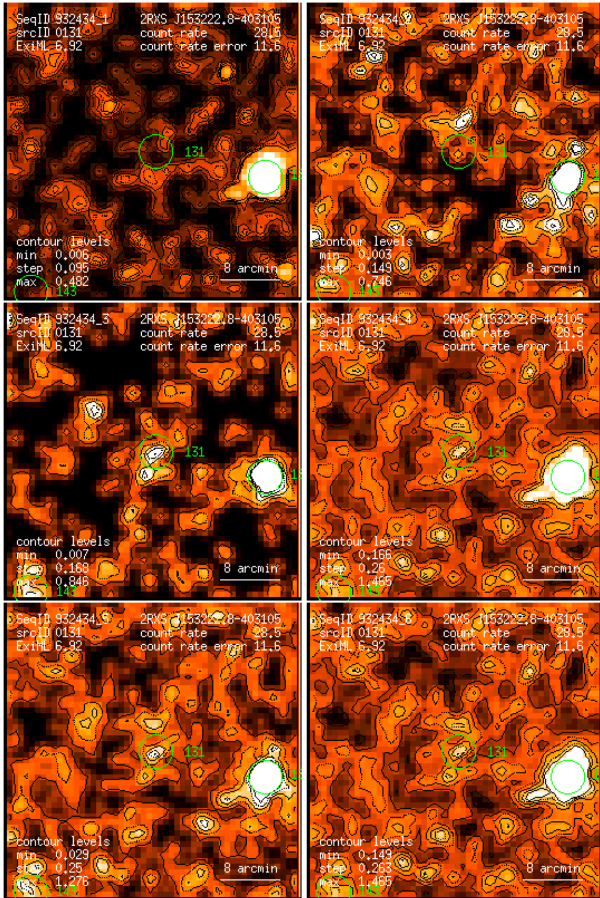
Figure 131: RASS 932434: detection 0131: band rate images, Gaussian filter: (1) PSPC channels 11 – 41, (2) 52 – 90, (3) 91 – 201, (4) 11 – 235, (5) 52 – 201, (6) 11 – 201. Broad band rates in counts/ks. Band rate contour levels in counts/ks/arcmin 2 .
