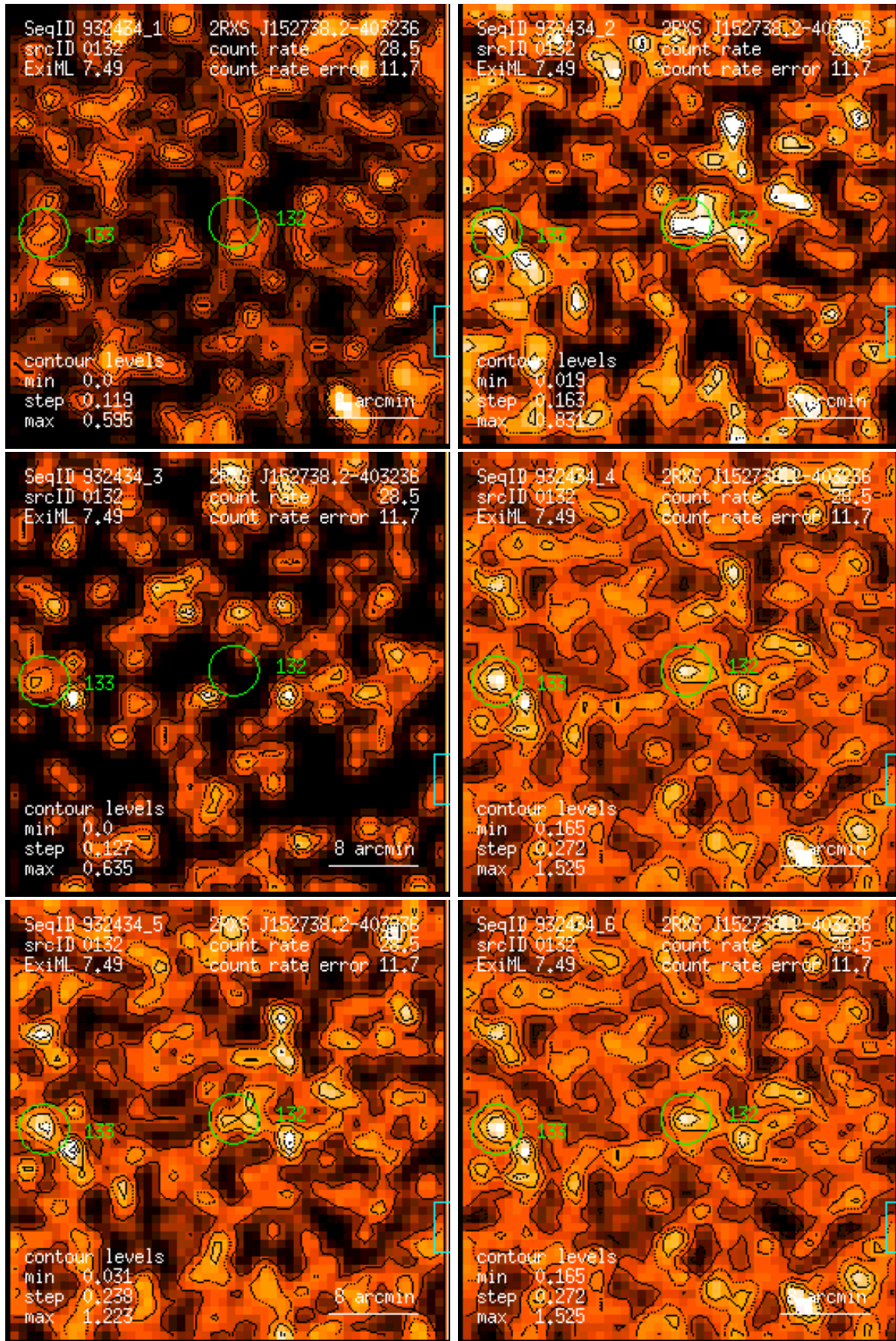
Figure 132: RASS 932434: detection 0132: band rate images, Gaussian filter: (1) PSPC channels 11 – 41, (2) 52 – 90, (3) 91 – 201, (4) 11 – 235, (5) 52 – 201, (6) 11 – 201. Broad band rates in counts/ks. Band rate contour levels in counts/ks/arcmin 2 .
