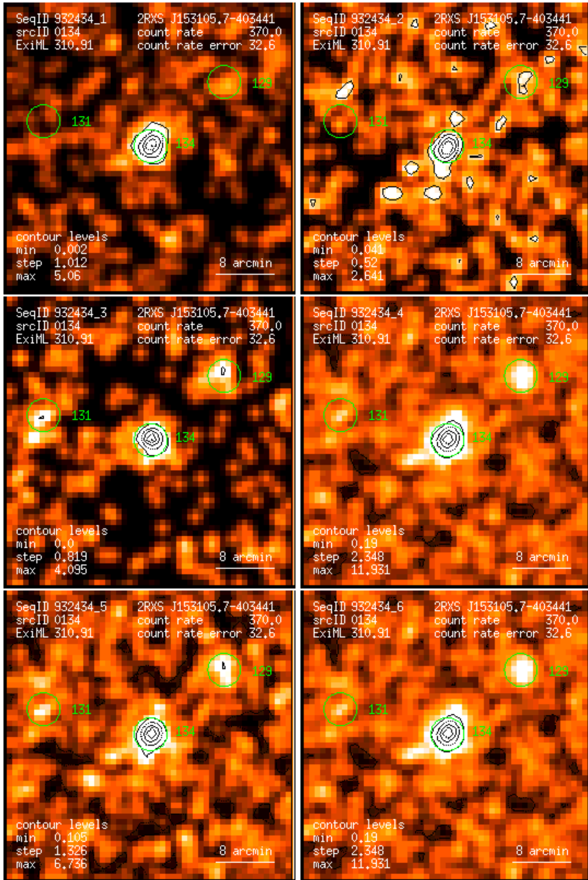
Figure 134: RASS 932434: detection 0134: band rate images, Gaussian filter: (1) PSPC channels 11 – 41, (2) 52 – 90, (3) 91 – 201, (4) 11 – 235, (5) 52 – 201, (6) 11 – 201. Broad band rates in counts/ks. Band rate contour levels in counts/ks/arcmin 2 .
