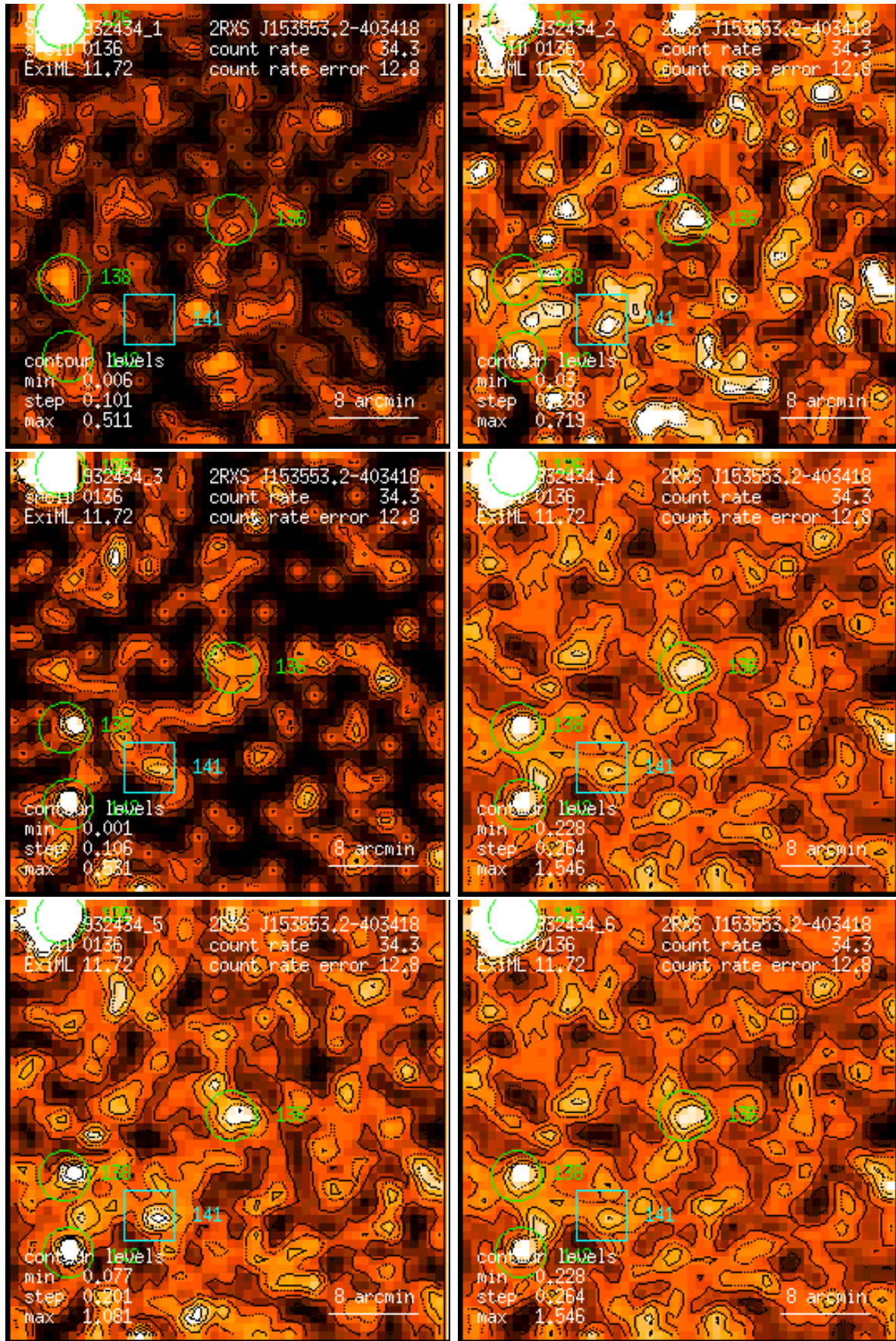
Figure 136: RASS 932434: detection 0136: band rate images, Gaussian filter: (1) PSPC channels 11 – 41, (2) 52 – 90, (3) 91 – 201, (4) 11 – 235, (5) 52 – 201, (6) 11 – 201. Broad band rates in counts/ks. Band rate contour levels in counts/ks/arcmin 2 .
