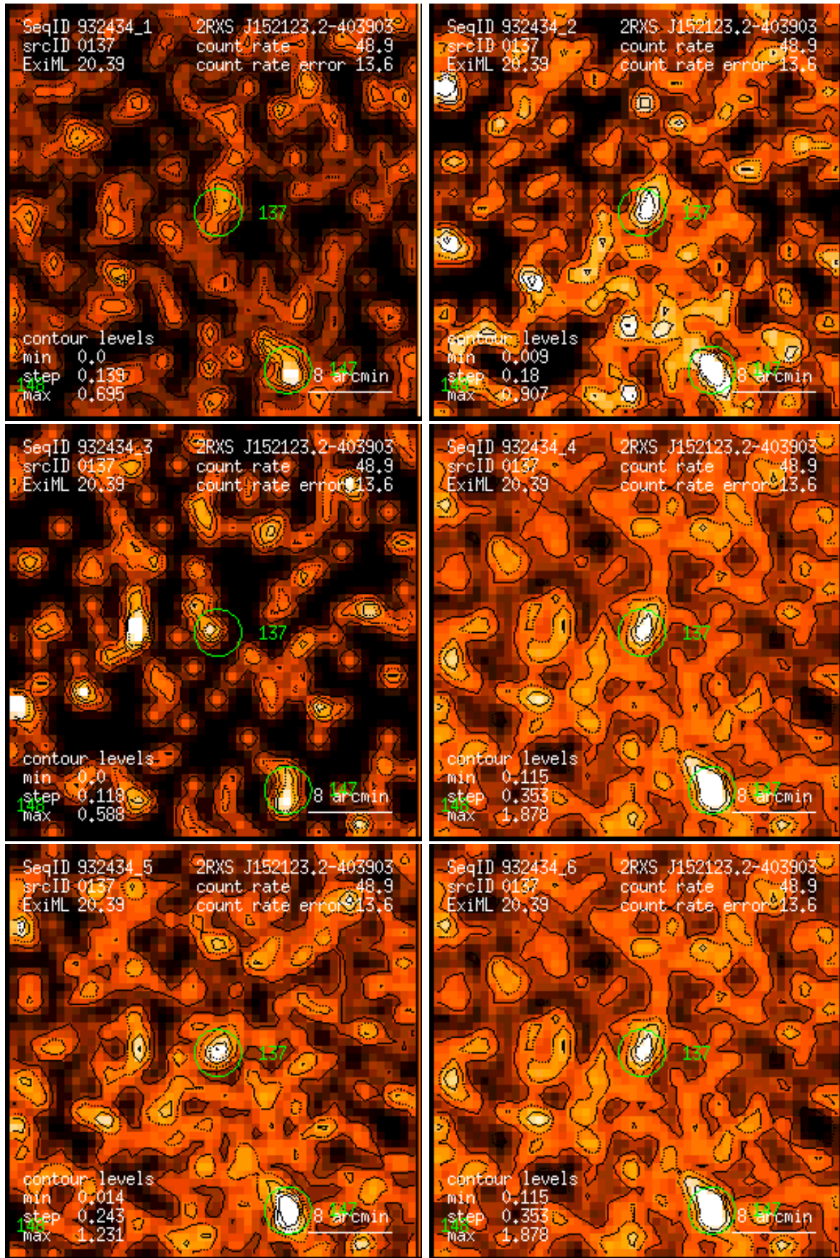
Figure 137: RASS 932434: detection 0137: band rate images, Gaussian filter: (1) PSPC channels 11 – 41, (2) 52 – 90, (3) 91 – 201, (4) 11 – 235, (5) 52 – 201, (6) 11 – 201. Broad band rates in counts/ks. Band rate contour levels in counts/ks/arcmin 2 .
