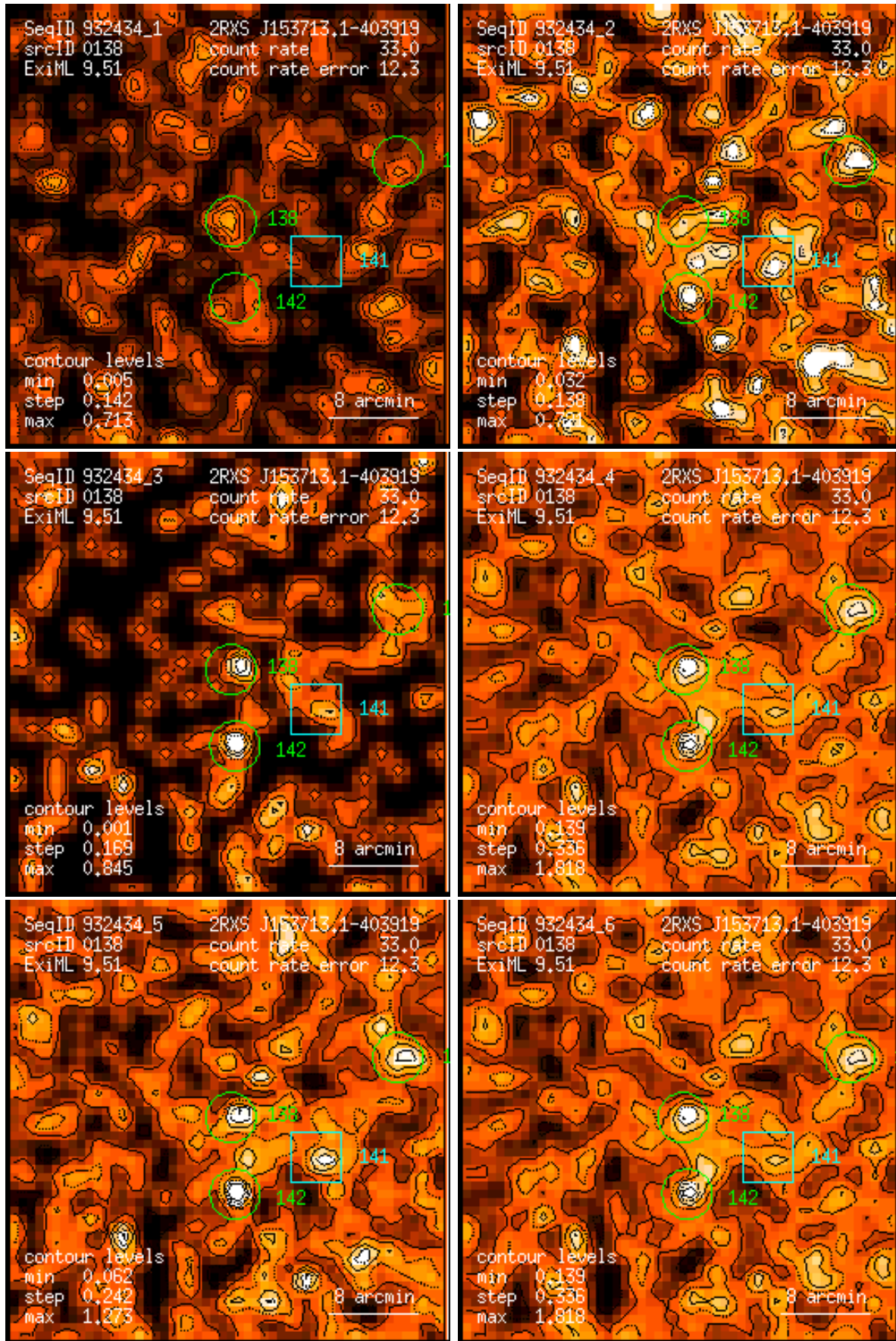
Figure 138: RASS 932434: detection 0138: band rate images, Gaussian filter: (1) PSPC channels 11 – 41, (2) 52 – 90, (3) 91 – 201, (4) 11 – 235, (5) 52 – 201, (6) 11 – 201. Broad band rates in counts/ks. Band rate contour levels in counts/ks/arcmin 2 .
