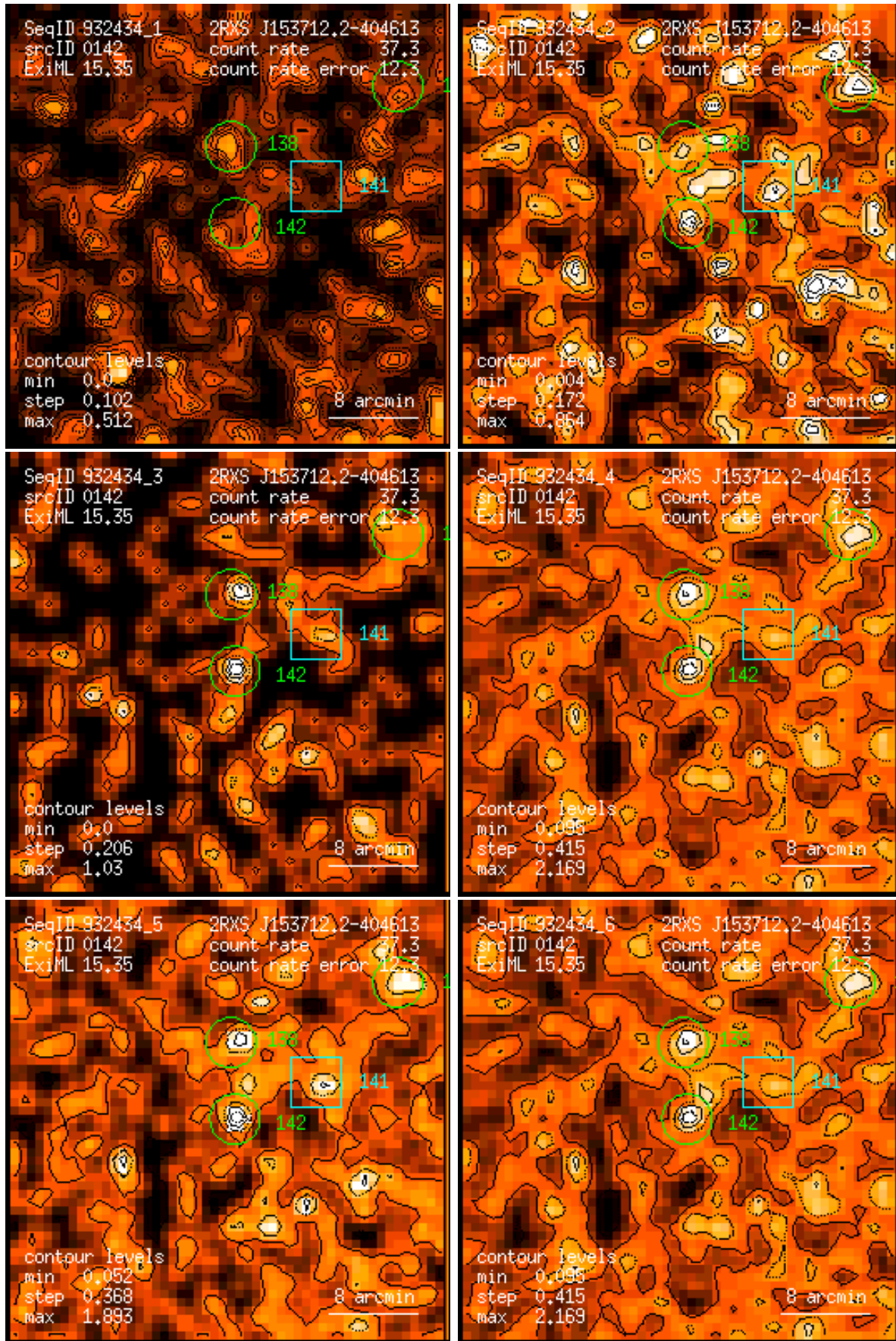
Figure 142: RASS 932434: detection 0142: band rate images, Gaussian filter: (1) PSPC channels 11 – 41, (2) 52 – 90, (3) 91 – 201, (4) 11 – 235, (5) 52 – 201, (6) 11 – 201. Broad band rates in counts/ks. Band rate contour levels in counts/ks/arcmin 2 .
