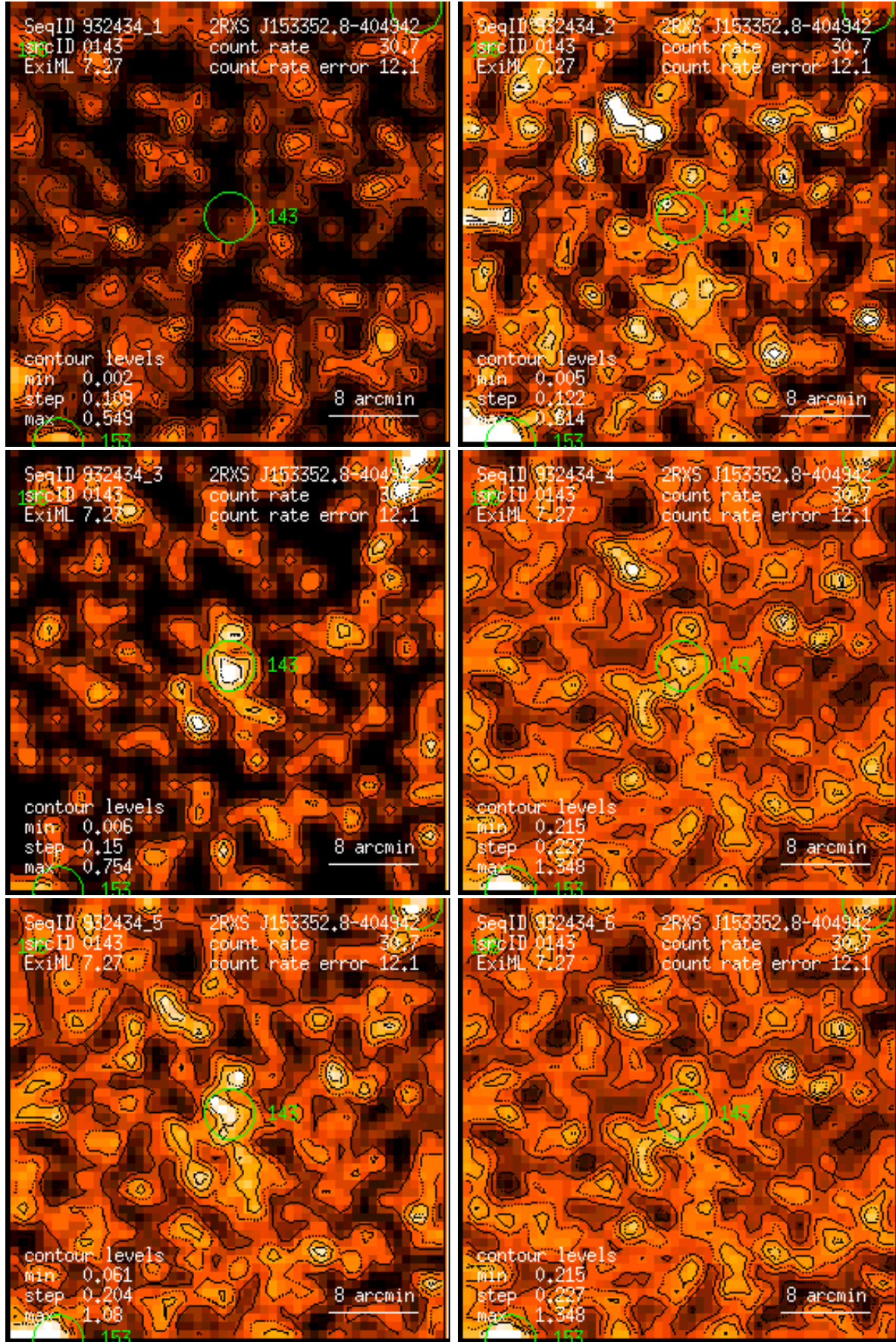
Figure 143: RASS 932434: detection 0143: band rate images, Gaussian filter: (1) PSPC channels 11 – 41, (2) 52 – 90, (3) 91 – 201, (4) 11 – 235, (5) 52 – 201, (6) 11 – 201. Broad band rates in counts/ks. Band rate contour levels in counts/ks/arcmin 2 .
