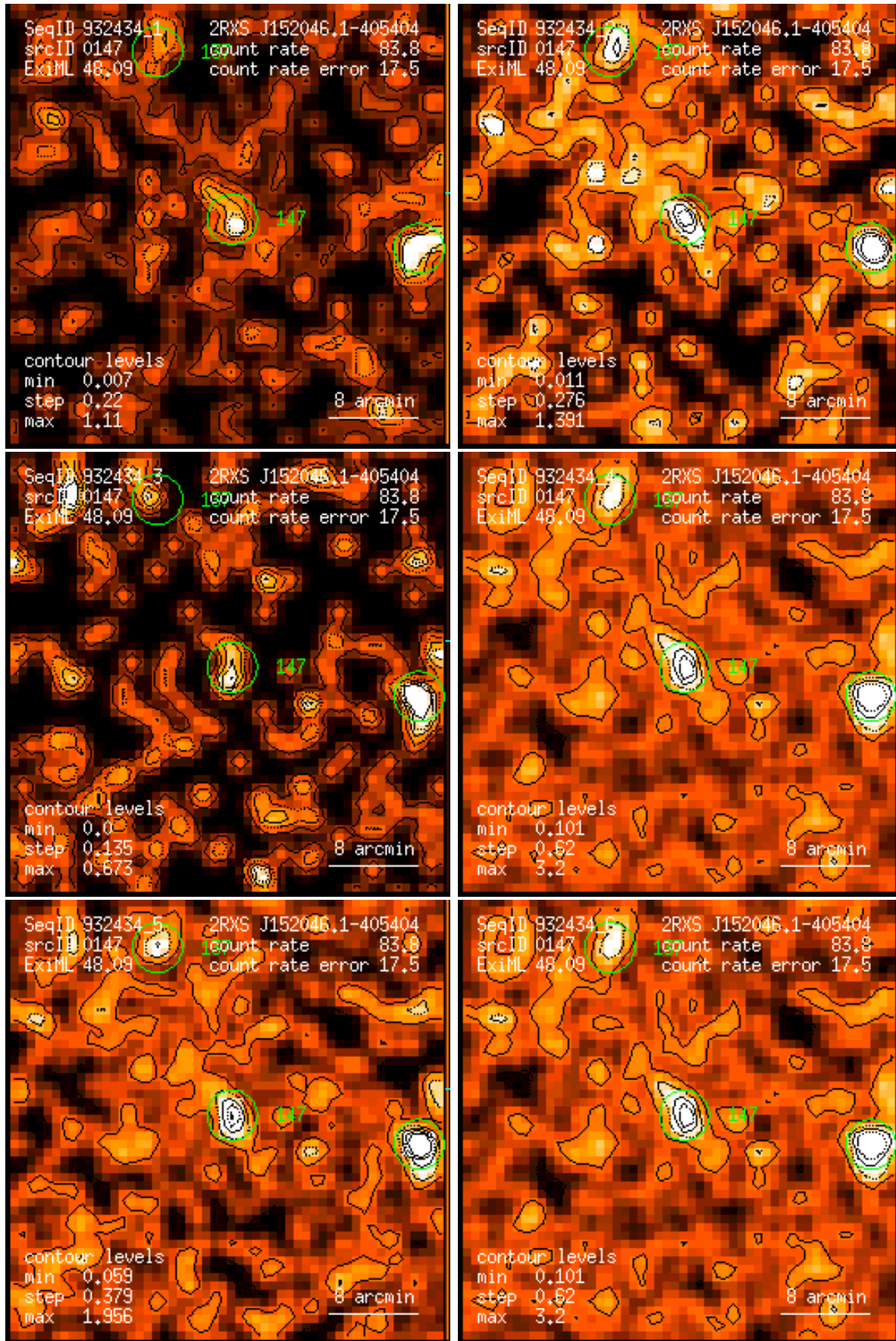
Figure 147: RASS 932434: detection 0147: band rate images, Gaussian filter: (1) PSPC channels 11 – 41, (2) 52 – 90, (3) 91 – 201, (4) 11 – 235, (5) 52 – 201, (6) 11 – 201. Broad band rates in counts/ks. Band rate contour levels in counts/ks/arcmin 2 .
