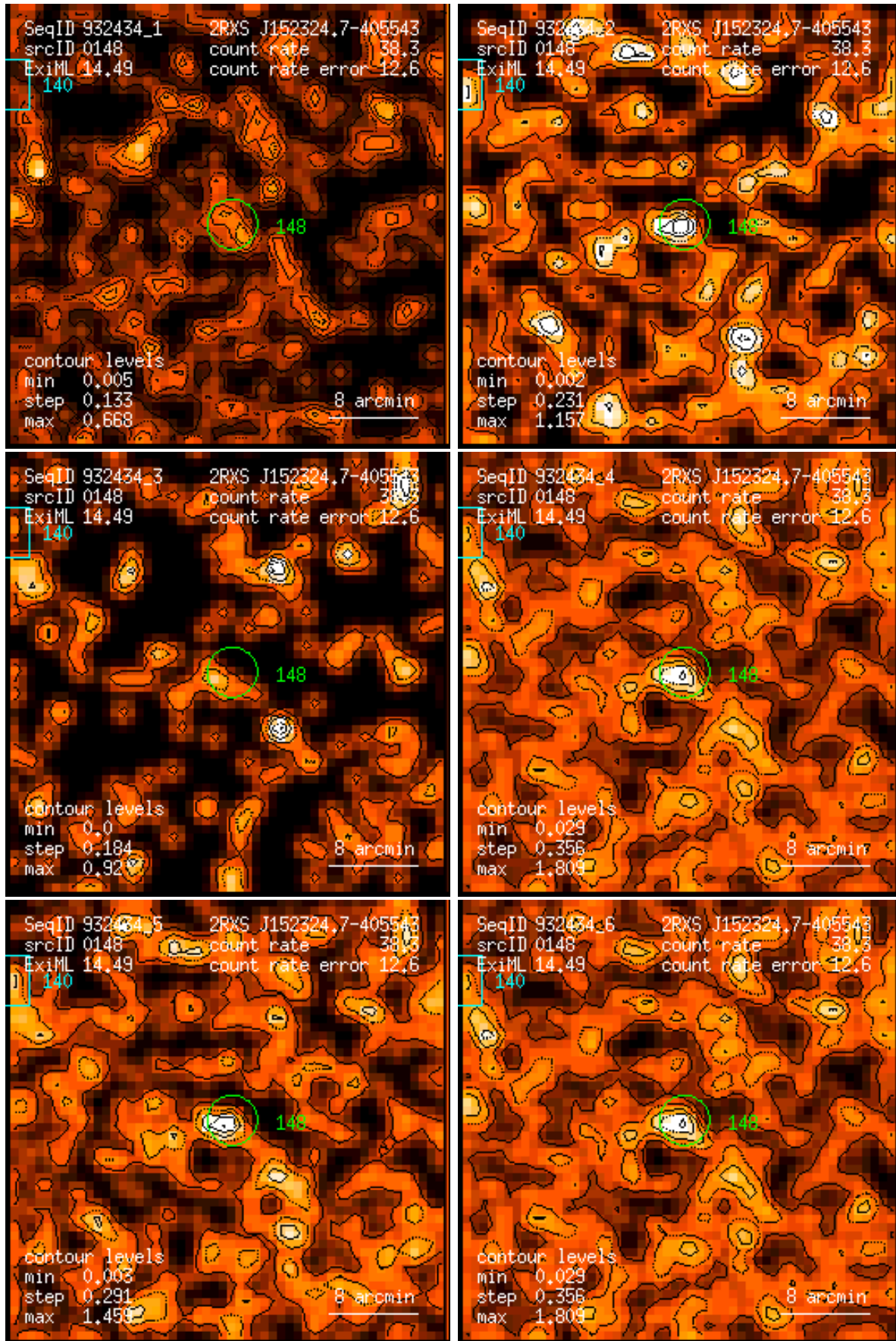
Figure 148: RASS 932434: detection 0148: band rate images, Gaussian filter: (1) PSPC channels 11 – 41, (2) 52 – 90, (3) 91 – 201, (4) 11 – 235, (5) 52 – 201, (6) 11 – 201. Broad band rates in counts/ks. Band rate contour levels in counts/ks/arcmin 2 .
