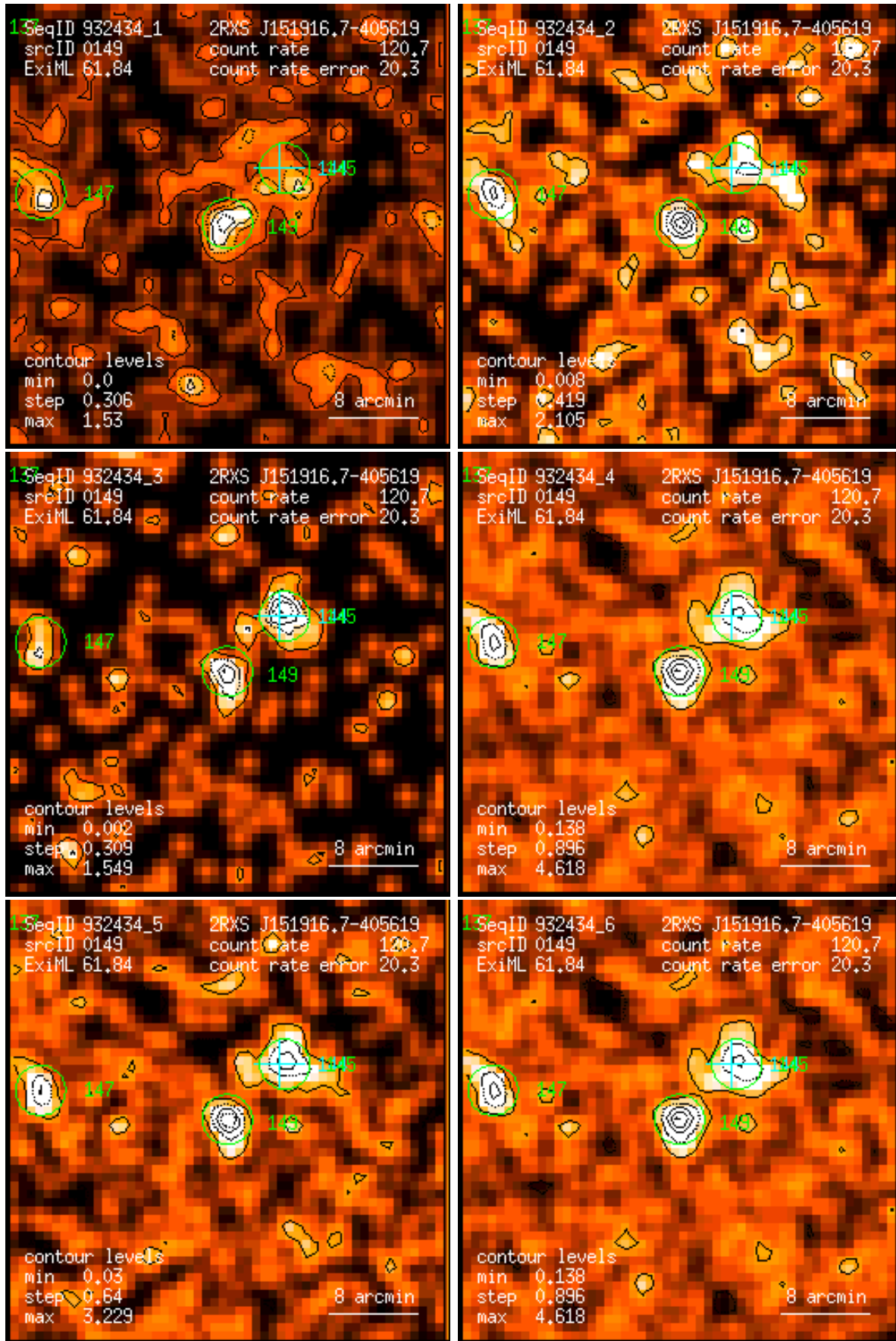
Figure 149: RASS 932434: detection 0149: band rate images, Gaussian filter: (1) PSPC channels 11 – 41, (2) 52 – 90, (3) 91 – 201, (4) 11 – 235, (5) 52 – 201, (6) 11 – 201. Broad band rates in counts/ks. Band rate contour levels in counts/ks/arcmin 2 .
