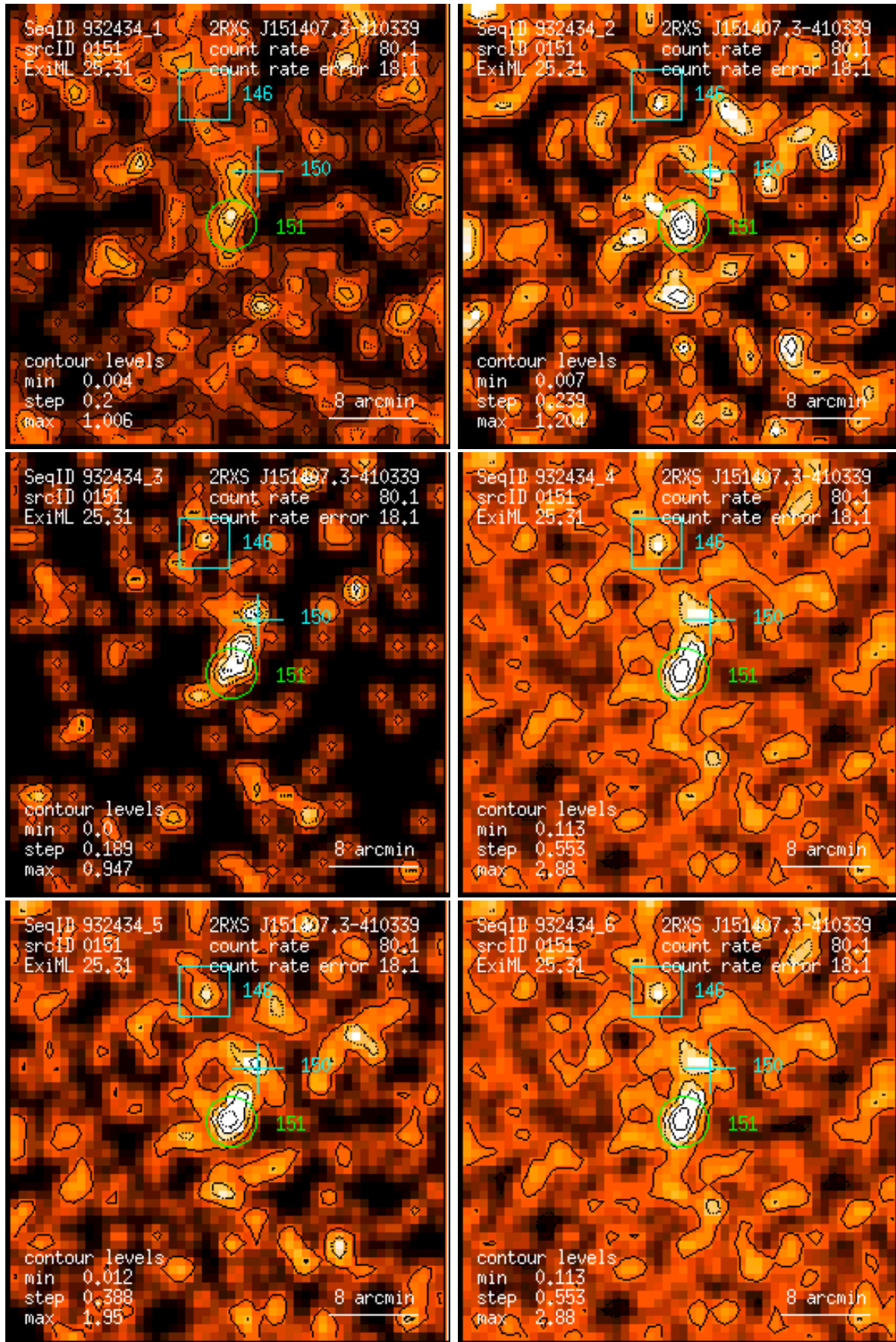
Figure 151: RASS 932434: detection 0151: band rate images, Gaussian filter: (1) PSPC channels 11 – 41, (2) 52 – 90, (3) 91 – 201, (4) 11 – 235, (5) 52 – 201, (6) 11 – 201. Broad band rates in counts/ks. Band rate contour levels in counts/ks/arcmin 2 .
