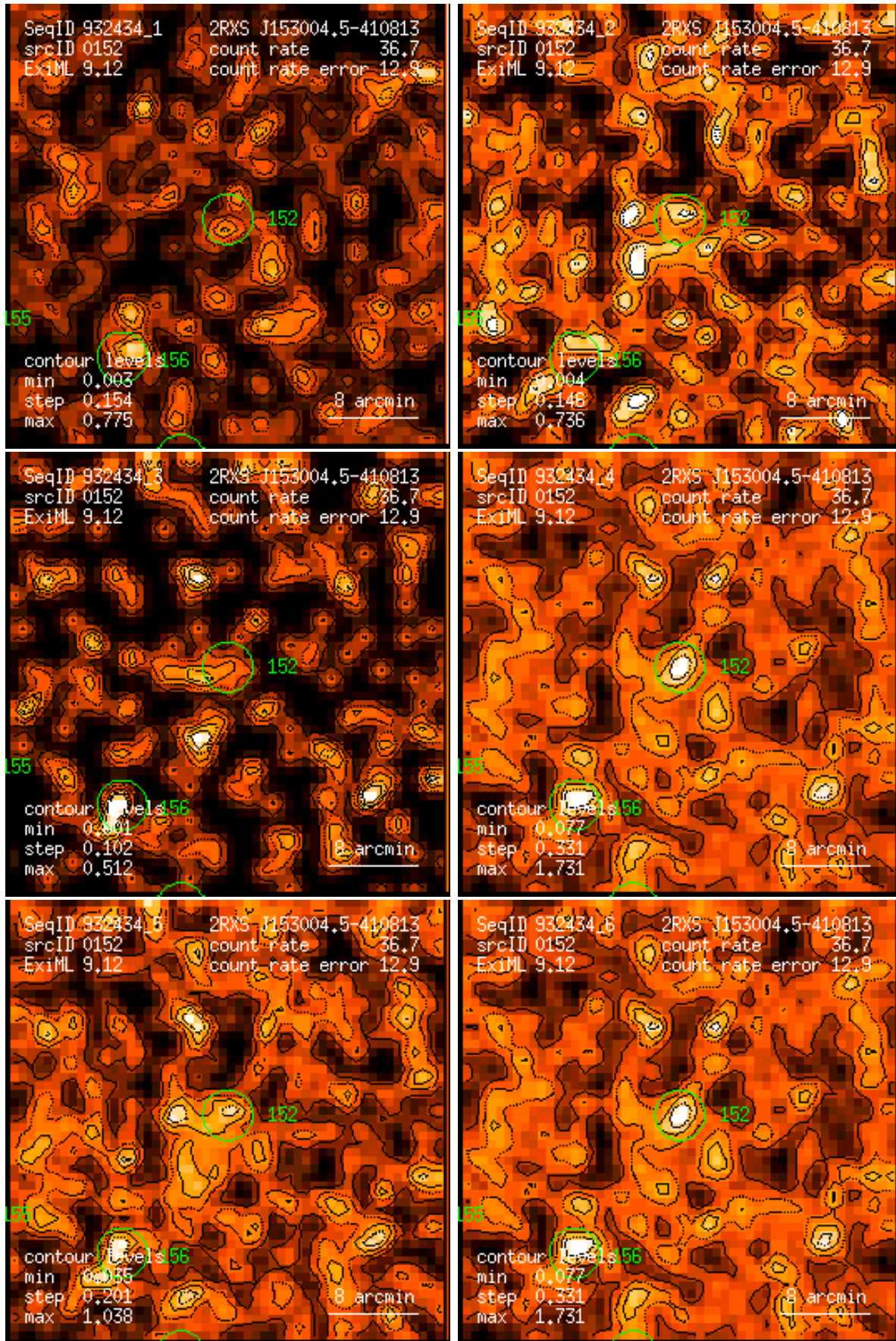
Figure 152: RASS 932434: detection 0152: band rate images, Gaussian filter: (1) PSPC channels 11 – 41, (2) 52 – 90, (3) 91 – 201, (4) 11 – 235, (5) 52 – 201, (6) 11 – 201. Broad band rates in counts/ks. Band rate contour levels in counts/ks/arcmin 2 .
