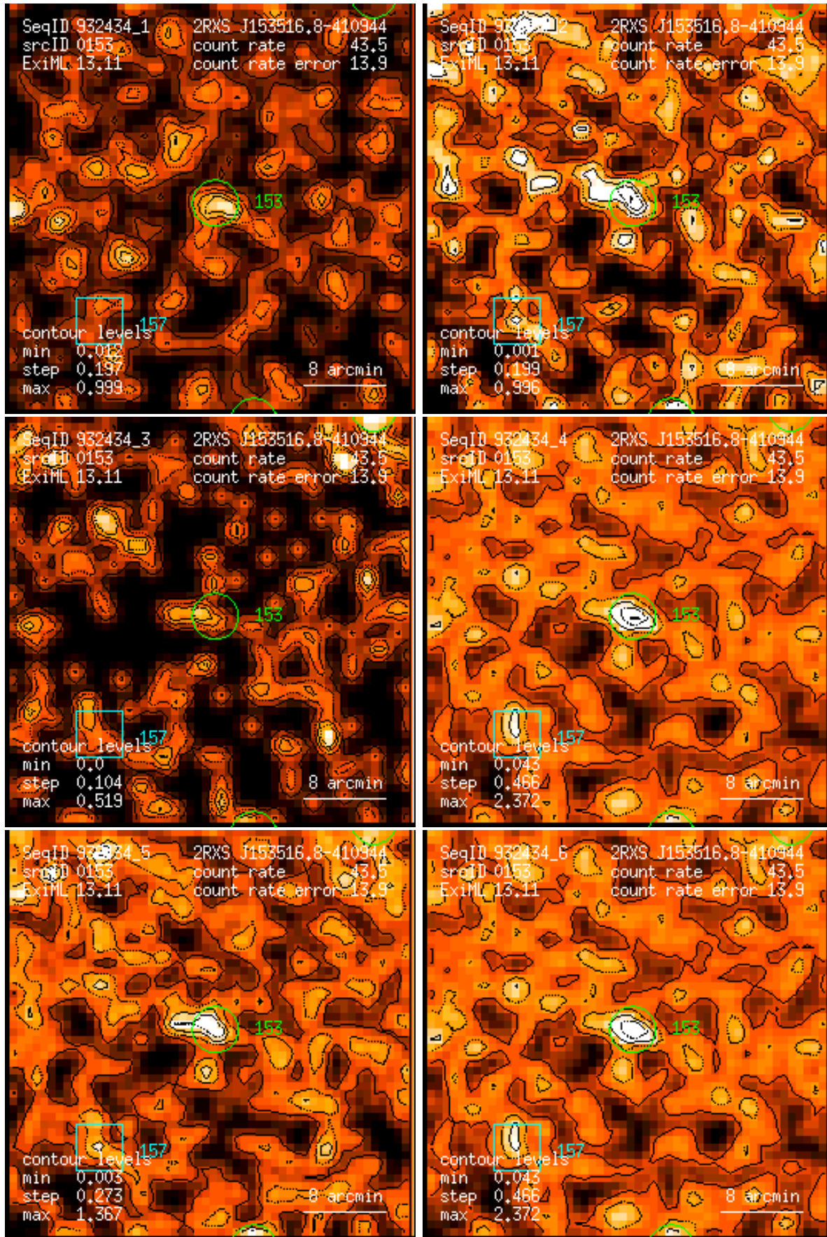
Figure 153: RASS 932434: detection 0153: band rate images, Gaussian filter: (1) PSPC channels 11 – 41, (2) 52 – 90, (3) 91 – 201, (4) 11 – 235, (5) 52 – 201, (6) 11 – 201. Broad band rates in counts/ks. Band rate contour levels in counts/ks/arcmin 2 .
