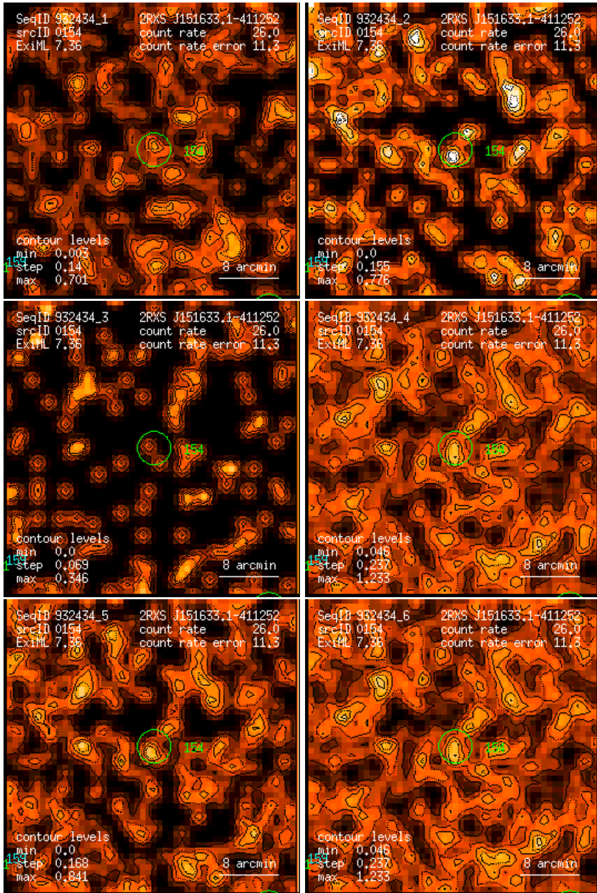
Figure 154: RASS 932434: detection 0154: band rate images, Gaussian filter: (1) PSPC channels 11 – 41, (2) 52 – 90, (3) 91 – 201, (4) 11 – 235, (5) 52 – 201, (6) 11 – 201. Broad band rates in counts/ks. Band rate contour levels in counts/ks/arcmin 2 .
