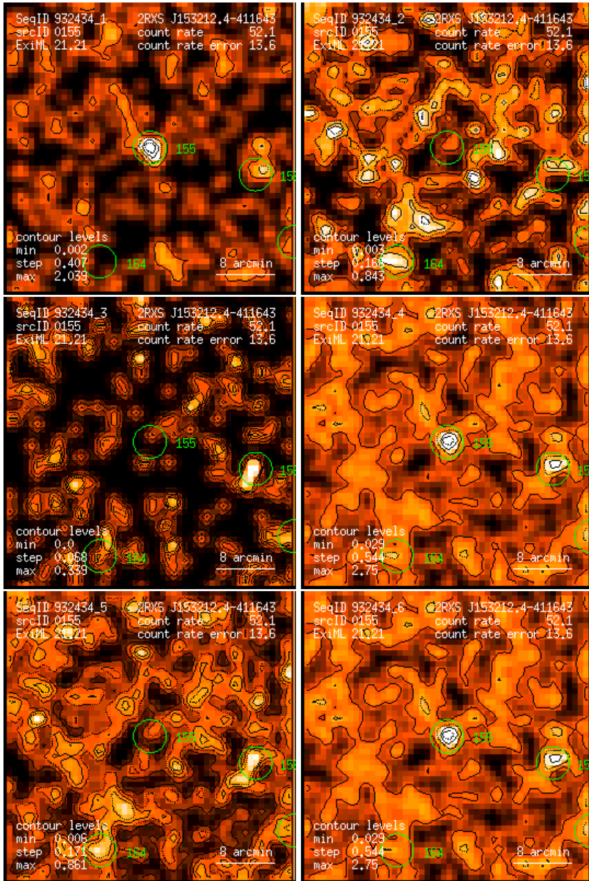
Figure 155: RASS 932434: detection 0155: band rate images, Gaussian filter: (1) PSPC channels 11 – 41, (2) 52 – 90, (3) 91 – 201, (4) 11 – 235, (5) 52 – 201, (6) 11 – 201. Broad band rates in counts/ks. Band rate contour levels in counts/ks/arcmin 2 .
