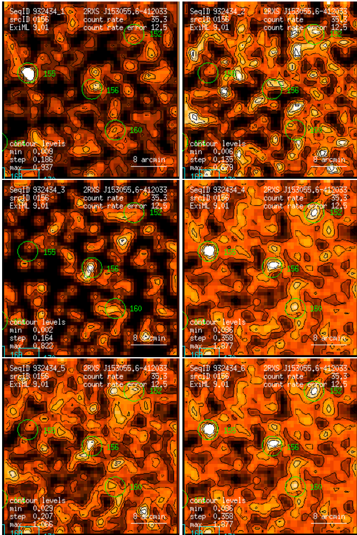
Figure 156: RASS 932434: detection 0156: band rate images, Gaussian filter: (1) PSPC channels 11 – 41, (2) 52 – 90, (3) 91 – 201, (4) 11 – 235, (5) 52 – 201, (6) 11 – 201. Broad band rates in counts/ks. Band rate contour levels in counts/ks/arcmin 2 .
