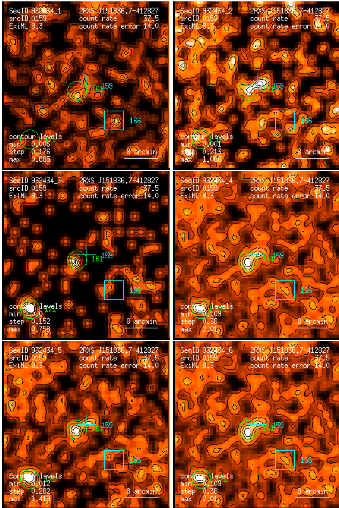
Figure 159: RASS 932434: detection 0159: band rate images, Gaussian filter: (1) PSPC channels 11 – 41, (2) 52 – 90, (3) 91 – 201, (4) 11 – 235, (5) 52 – 201, (6) 11 – 201. Broad band rates in counts/ks. Band rate contour levels in counts/ks/arcmin 2 .
