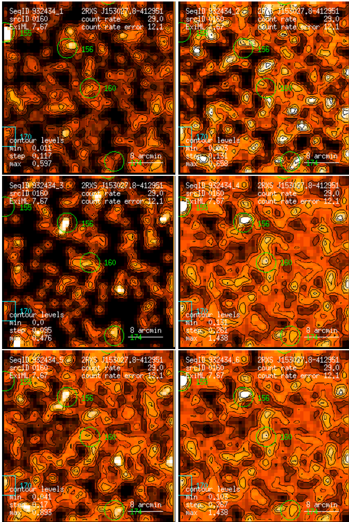
Figure 160: RASS 932434: detection 0160: band rate images, Gaussian filter: (1) PSPC channels 11 – 41, (2) 52 – 90, (3) 91 – 201, (4) 11 – 235, (5) 52 – 201, (6) 11 – 201. Broad band rates in counts/ks. Band rate contour levels in counts/ks/arcmin 2 .
