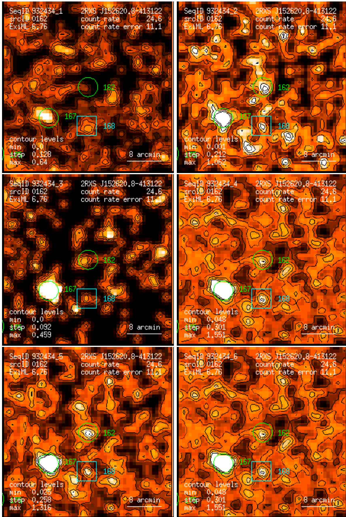
Figure 162: RASS 932434: detection 0162: band rate images, Gaussian filter: (1) PSPC channels 11 – 41, (2) 52 – 90, (3) 91 – 201, (4) 11 – 235, (5) 52 – 201, (6) 11 – 201. Broad band rates in counts/ks. Band rate contour levels in counts/ks/arcmin 2 .
