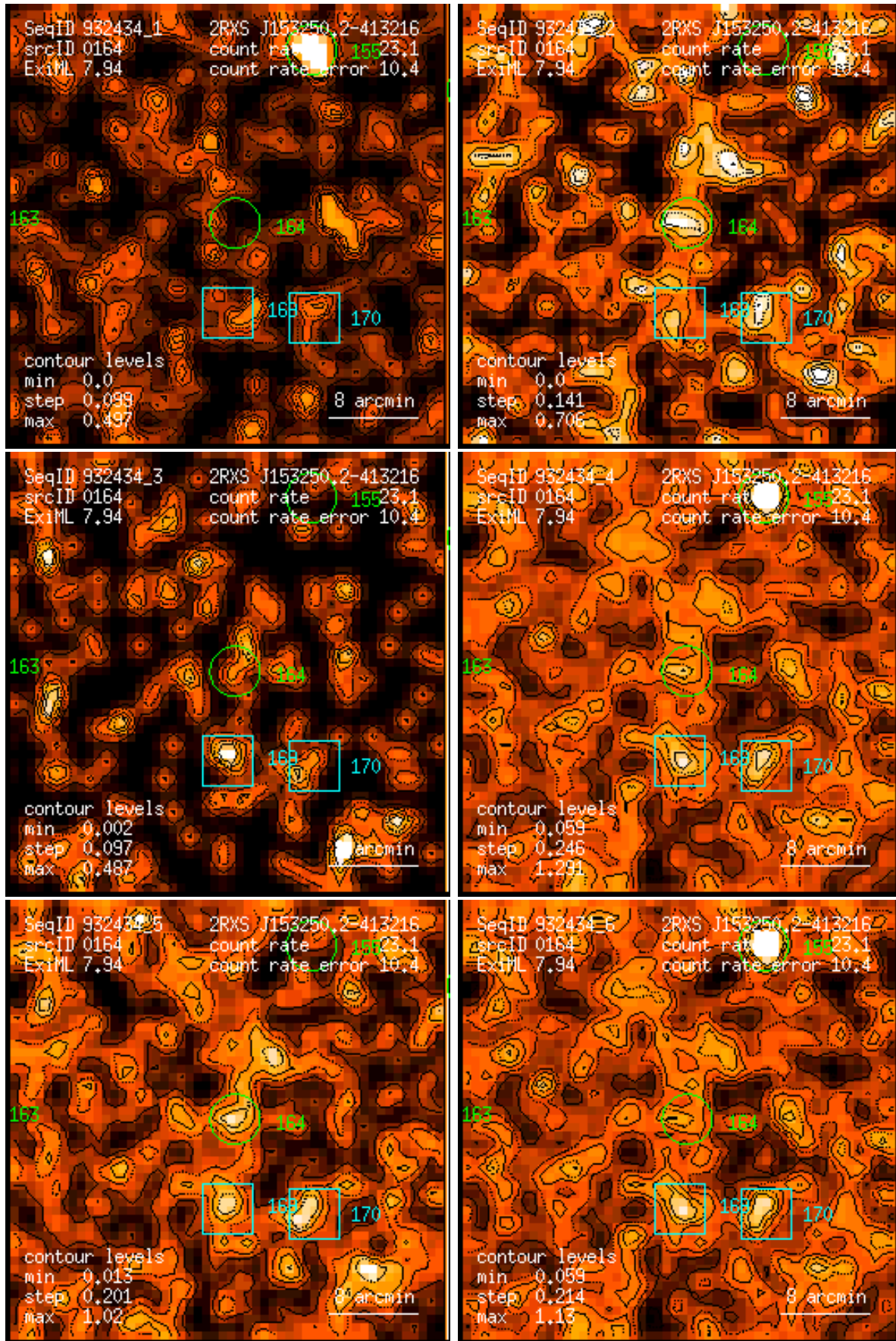
Figure 164: RASS 932434: detection 0164: band rate images, Gaussian filter: (1) PSPC channels 11 – 41, (2) 52 – 90, (3) 91 – 201, (4) 11 – 235, (5) 52 – 201, (6) 11 – 201. Broad band rates in counts/ks. Band rate contour levels in counts/ks/arcmin 2 .
