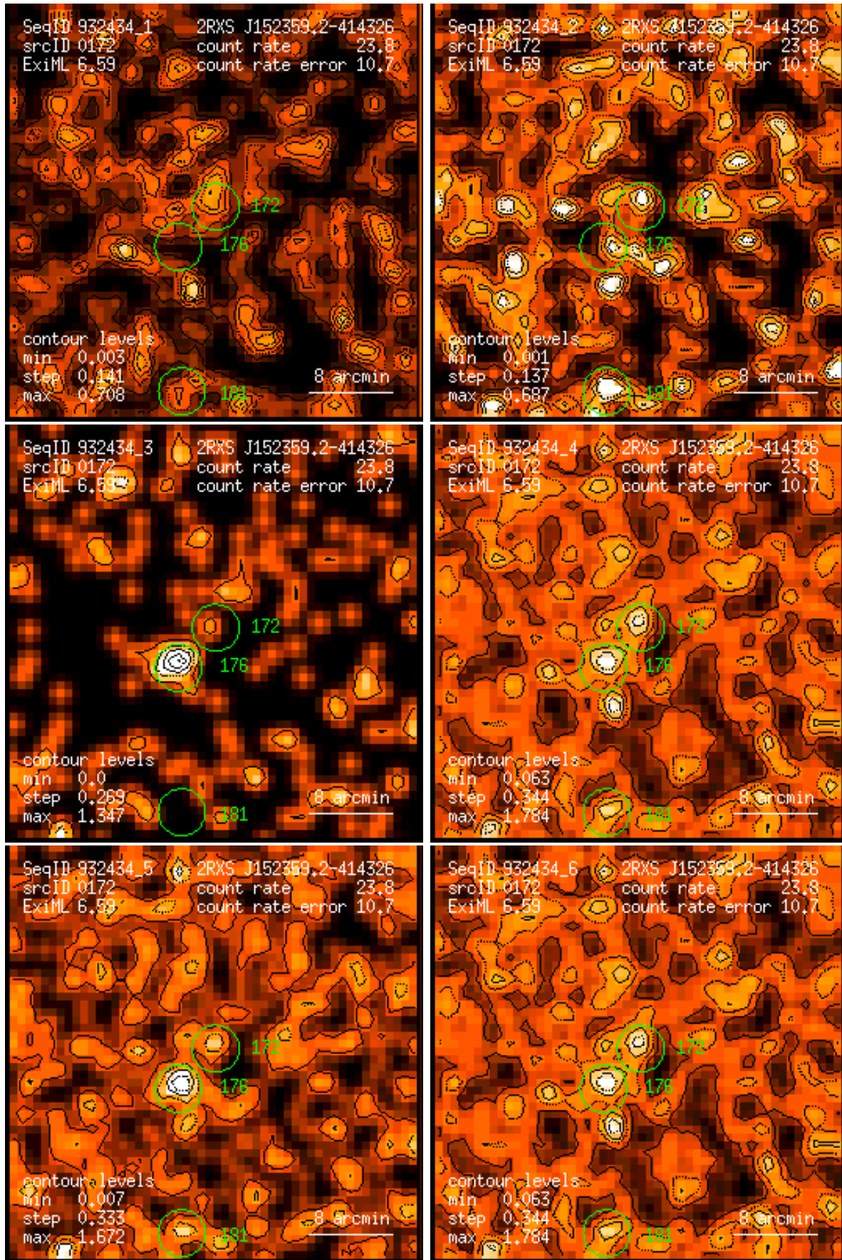
Figure 172: RASS 932434: detection 0172: band rate images, Gaussian filter: (1) PSPC channels 11 – 41, (2) 52 – 90, (3) 91 – 201, (4) 11 – 235, (5) 52 – 201, (6) 11 – 201. Broad band rates in counts/ks. Band rate contour levels in counts/ks/arcmin 2 .
