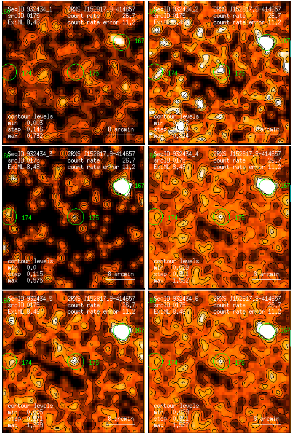
Figure 175: RASS 932434: detection 0175: band rate images, Gaussian filter: (1) PSPC channels 11 – 41, (2) 52 – 90, (3) 91 – 201, (4) 11 – 235, (5) 52 – 201, (6) 11 – 201. Broad band rates in counts/ks. Band rate contour levels in counts/ks/arcmin 2 .
