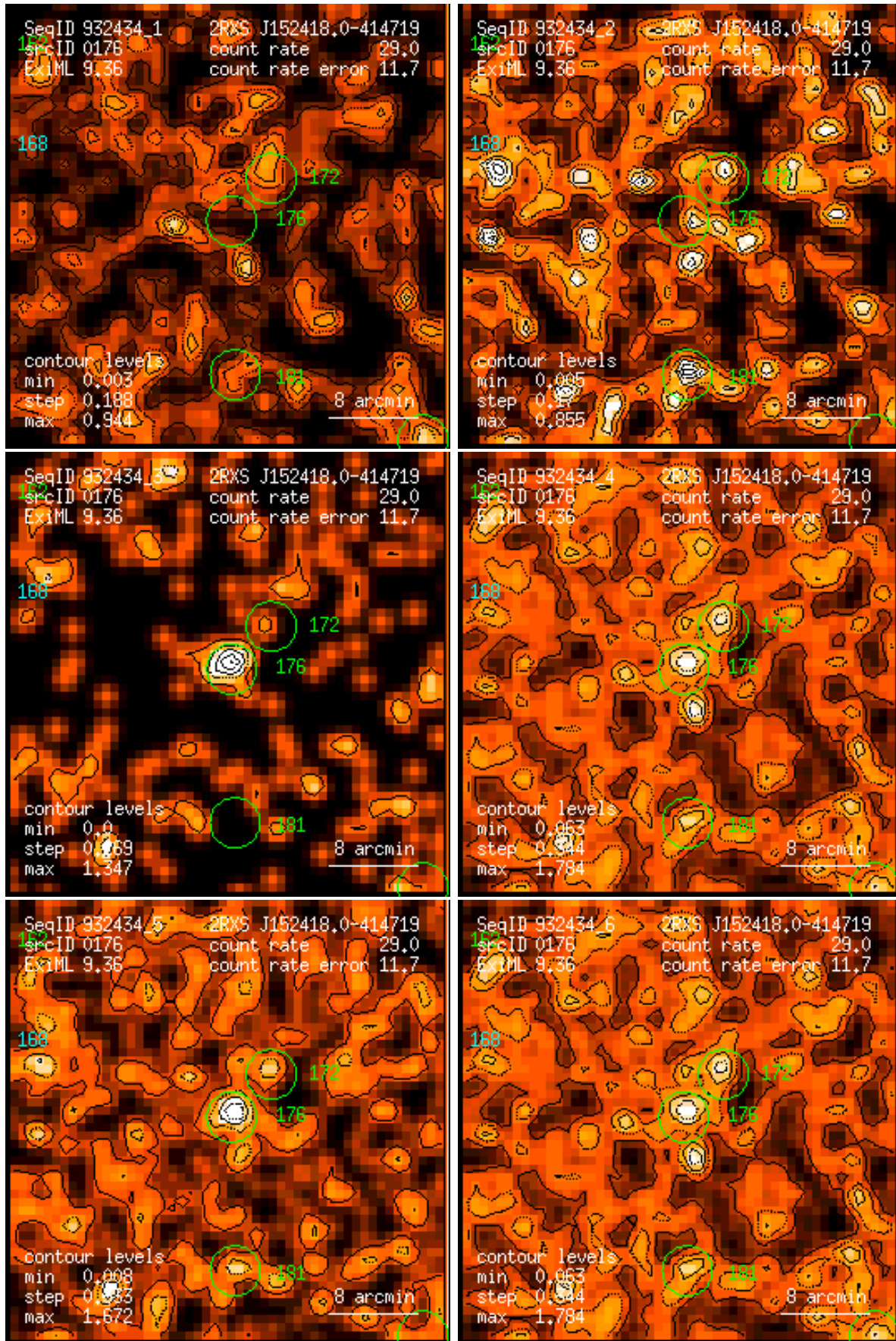
Figure 176: RASS 932434: detection 0176: band rate images, Gaussian filter: (1) PSPC channels 11 – 41, (2) 52 – 90, (3) 91 – 201, (4) 11 – 235, (5) 52 – 201, (6) 11 – 201. Broad band rates in counts/ks. Band rate contour levels in counts/ks/arcmin 2 .
