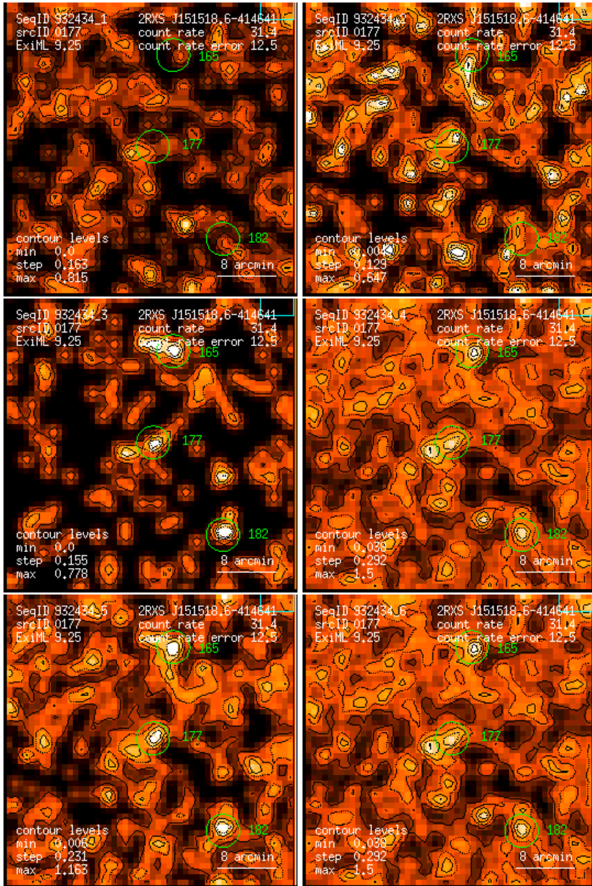
Figure 177: RASS 932434: detection 0177: band rate images, Gaussian filter: (1) PSPC channels 11 – 41, (2) 52 – 90, (3) 91 – 201, (4) 11 – 235, (5) 52 – 201, (6) 11 – 201. Broad band rates in counts/ks. Band rate contour levels in counts/ks/arcmin 2 .
