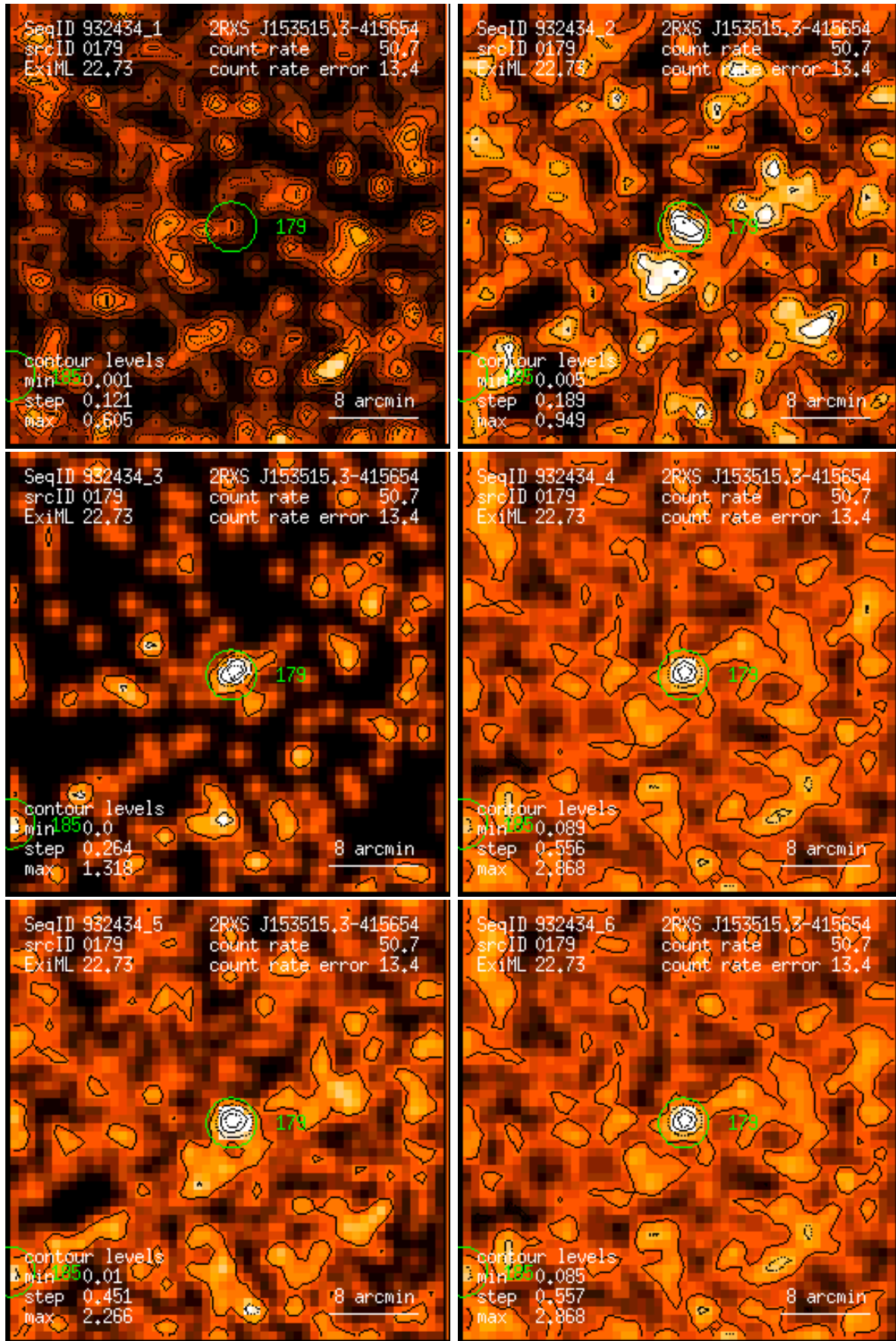
Figure 179: RASS 932434: detection 0179: band rate images, Gaussian filter: (1) PSPC channels 11 – 41, (2) 52 – 90, (3) 91 – 201, (4) 11 – 235, (5) 52 – 201, (6) 11 – 201. Broad band rates in counts/ks. Band rate contour levels in counts/ks/arcmin 2 .
