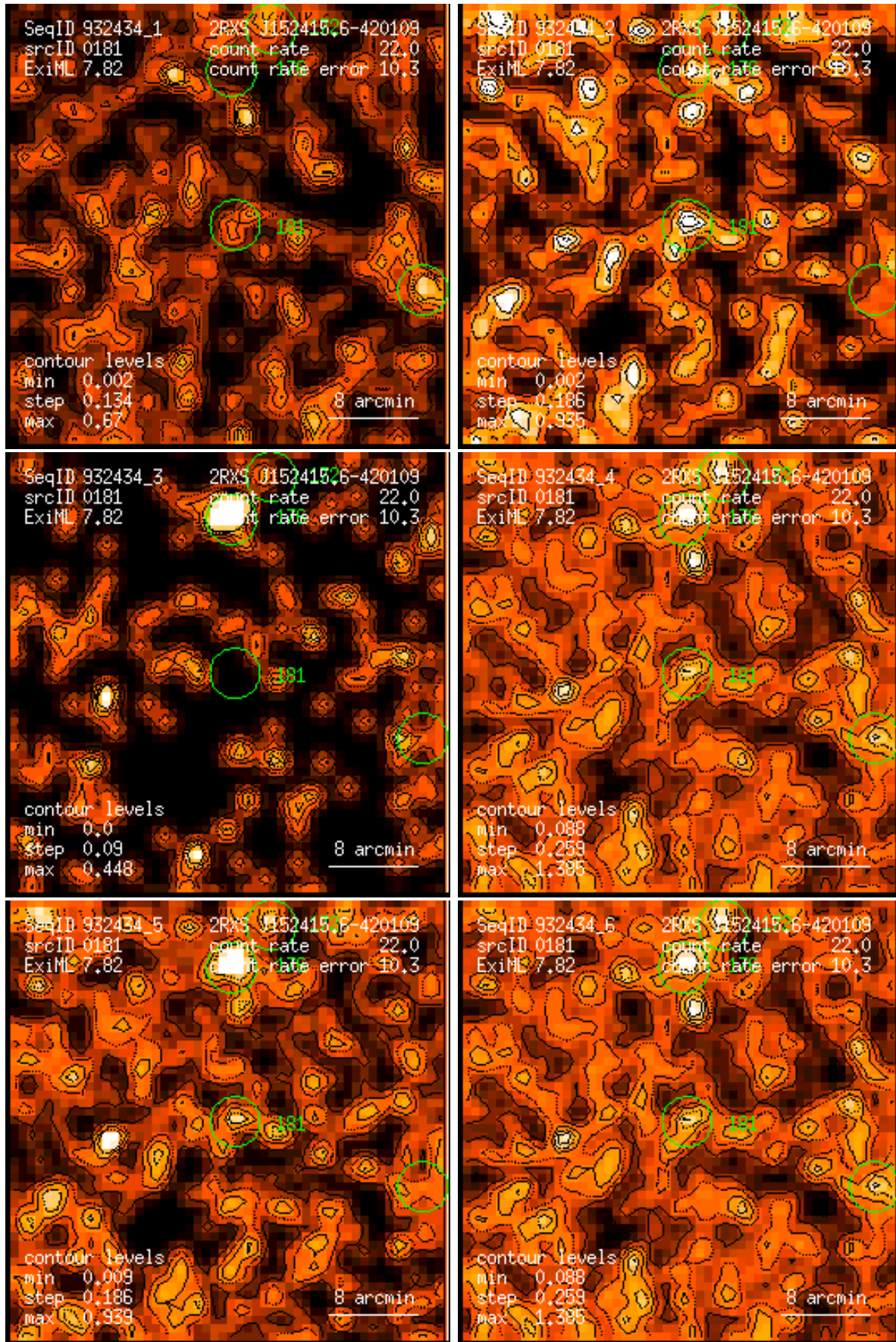
Figure 181: RASS 932434: detection 0181: band rate images, Gaussian filter: (1) PSPC channels 11 – 41, (2) 52 – 90, (3) 91 – 201, (4) 11 – 235, (5) 52 – 201, (6) 11 – 201. Broad band rates in counts/ks. Band rate contour levels in counts/ks/arcmin 2 .
