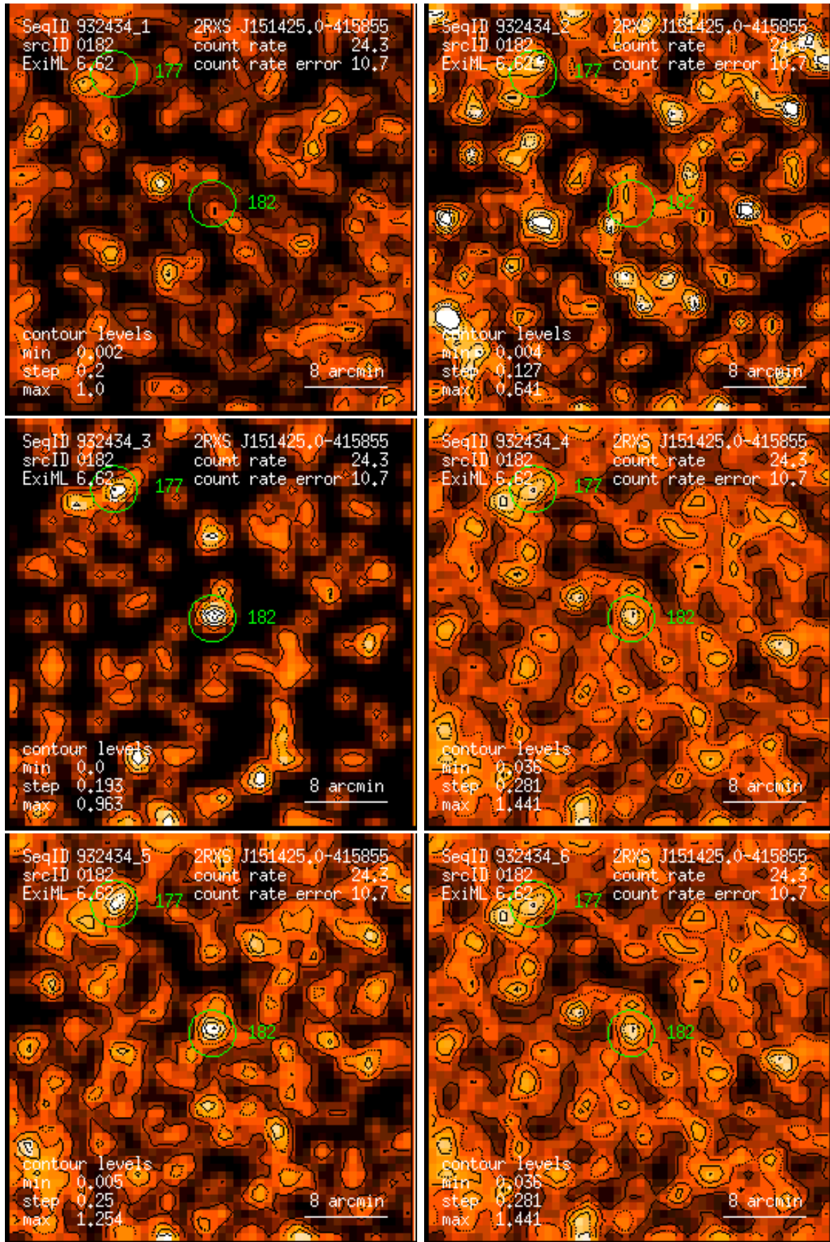
Figure 182: RASS 932434: detection 0182: band rate images, Gaussian filter: (1) PSPC channels 11 – 41, (2) 52 – 90, (3) 91 – 201, (4) 11 – 235, (5) 52 – 201, (6) 11 – 201. Broad band rates in counts/ks. Band rate contour levels in counts/ks/arcmin 2 .
