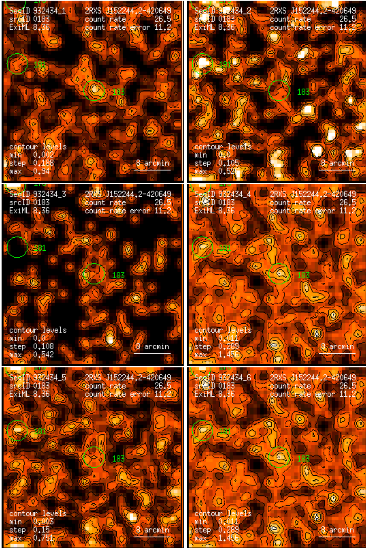
Figure 183: RASS 932434: detection 0183: band rate images, Gaussian filter: (1) PSPC channels 11 – 41, (2) 52 – 90, (3) 91 – 201, (4) 11 – 235, (5) 52 – 201, (6) 11 – 201. Broad band rates in counts/ks. Band rate contour levels in counts/ks/arcmin 2 .
