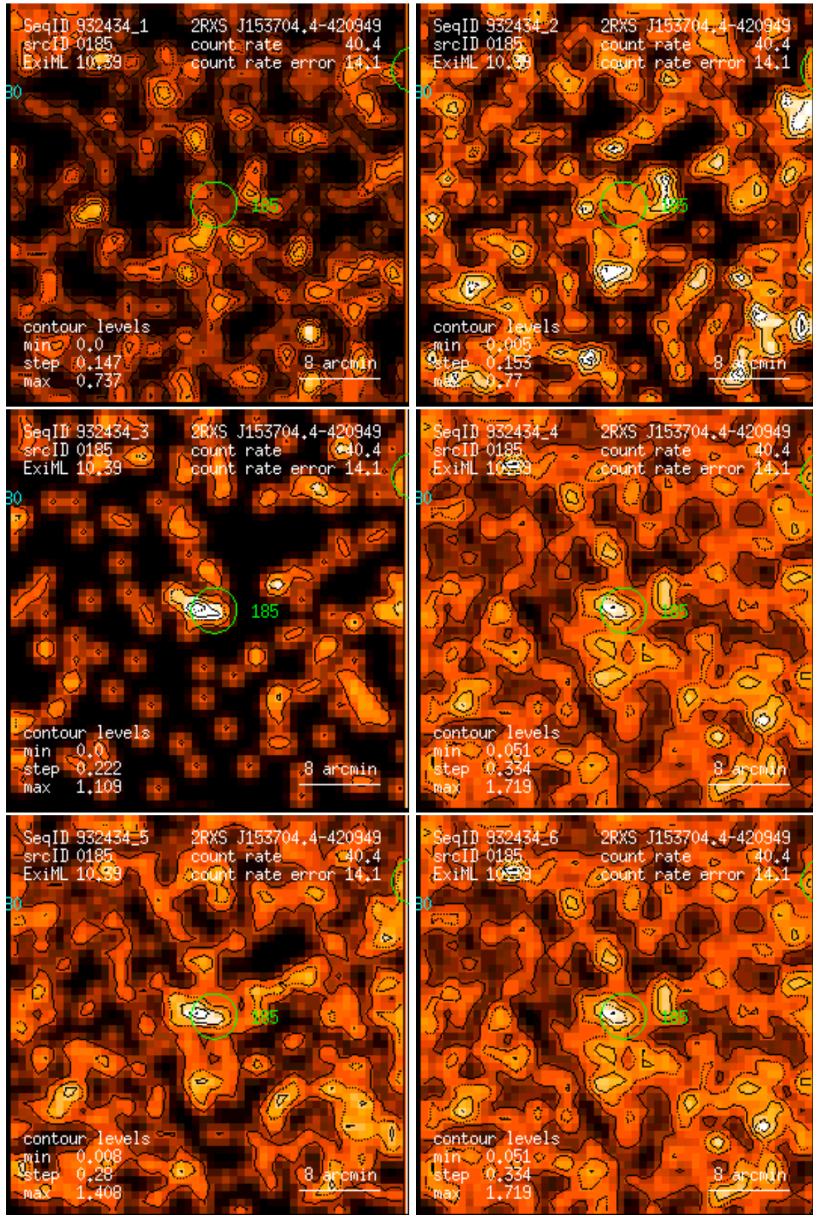
Figure 185: RASS 932434: detection 0185: band rate images, Gaussian filter: (1) PSPC channels 11 – 41, (2) 52 – 90, (3) 91 – 201, (4) 11 – 235, (5) 52 – 201, (6) 11 – 201. Broad band rates in counts/ks. Band rate contour levels in counts/ks/arcmin 2 .
