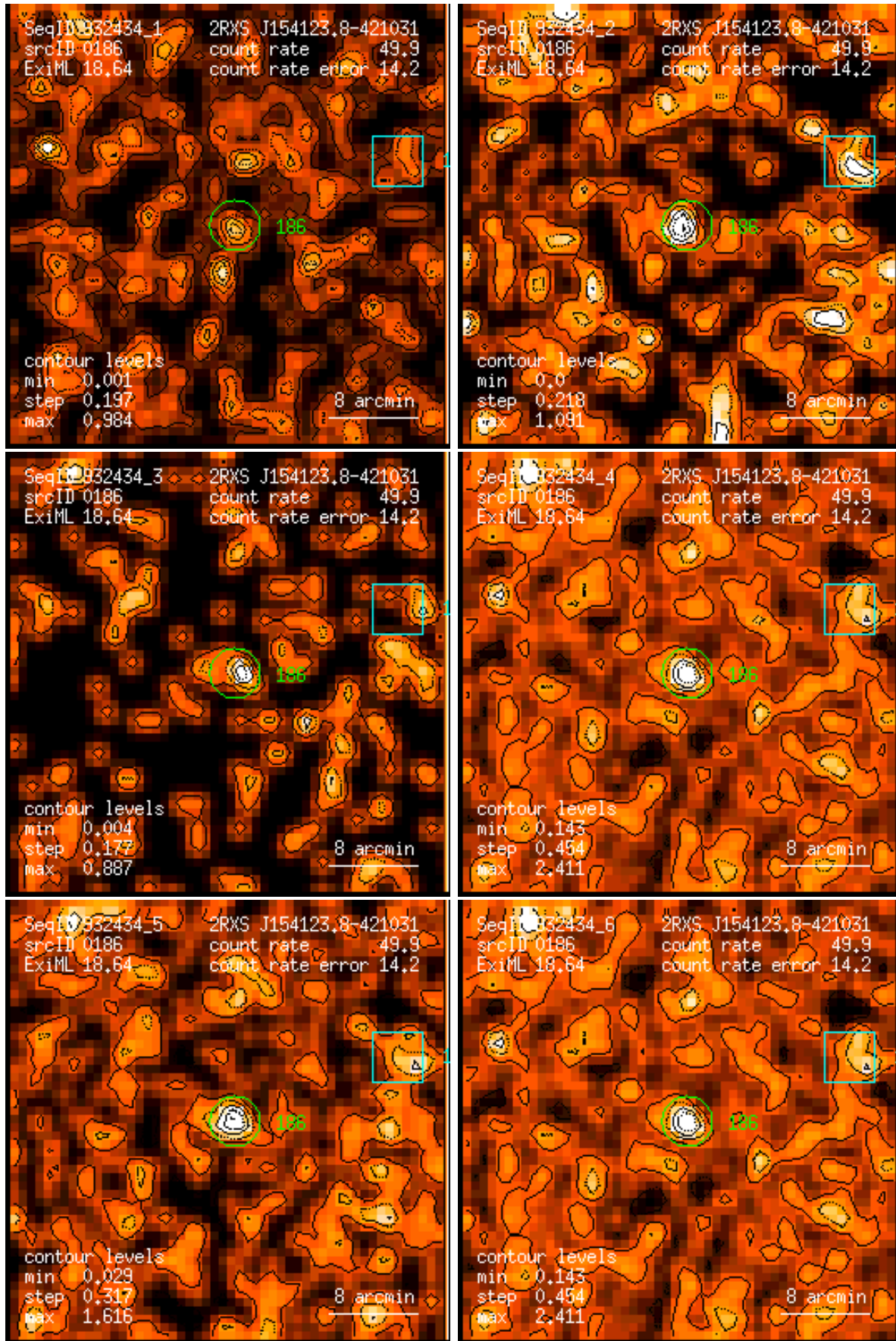
Figure 186: RASS 932434: detection 0186: band rate images, Gaussian filter: (1) PSPC channels 11 – 41, (2) 52 – 90, (3) 91 – 201, (4) 11 – 235, (5) 52 – 201, (6) 11 – 201. Broad band rates in counts/ks. Band rate contour levels in counts/ks/arcmin 2 .
